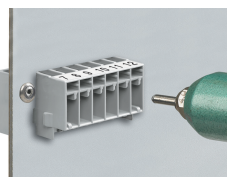
Mounting with 3 mm Ø blind rivets
