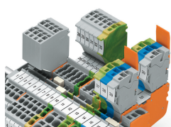
Female plugs can be individually locked.
