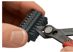
Coding a female connector by removing coding finger(s). (MCS MINI HD)
