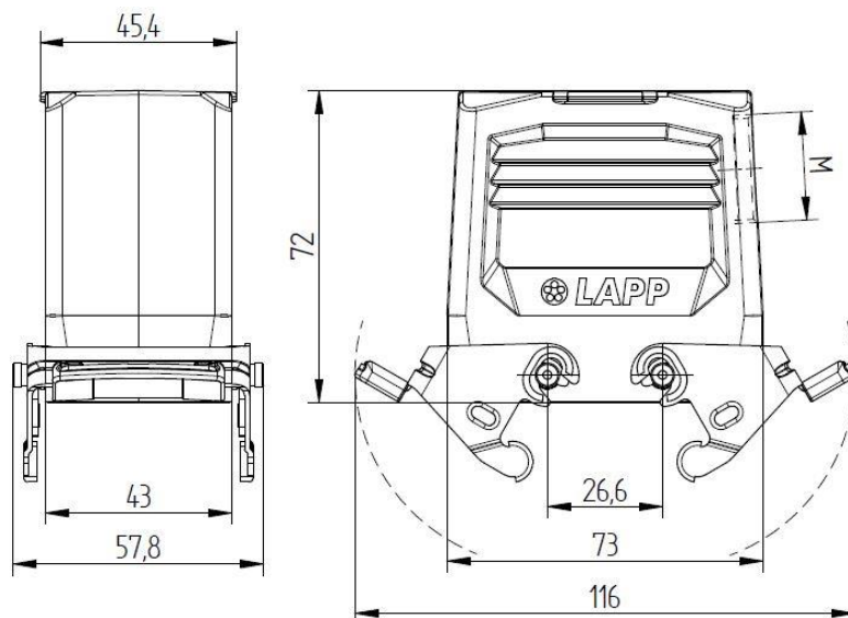
Side cable entry
