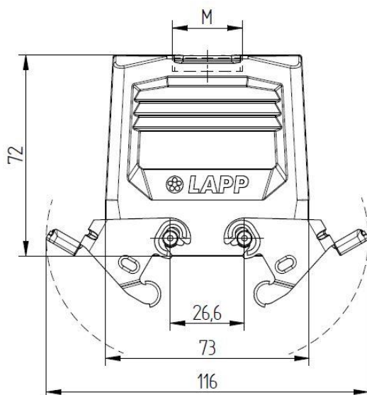
Top cable entry
