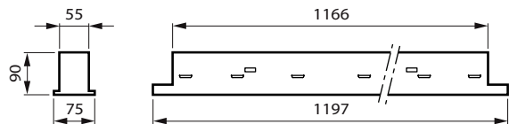
Recessed VPC_W8L120_sensor/IP
