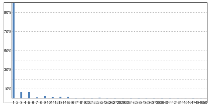
Current Harmonics %
