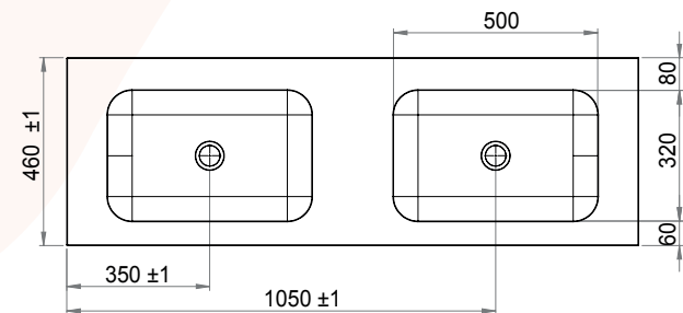
1400 mm double/left/right 2 laden | 2 drawers | 2 tiroirs
