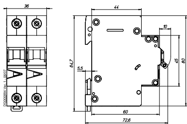
1+N-poles, 2-poles
