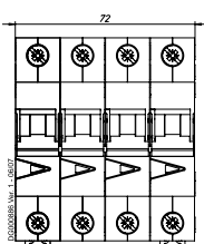
3+N-poles, 4-poles
