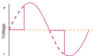
Forward-phase control dimmer
