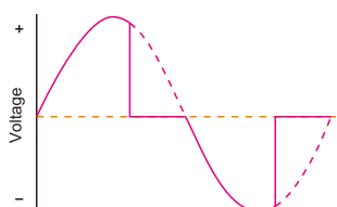
Reverse-phase control dimmer
