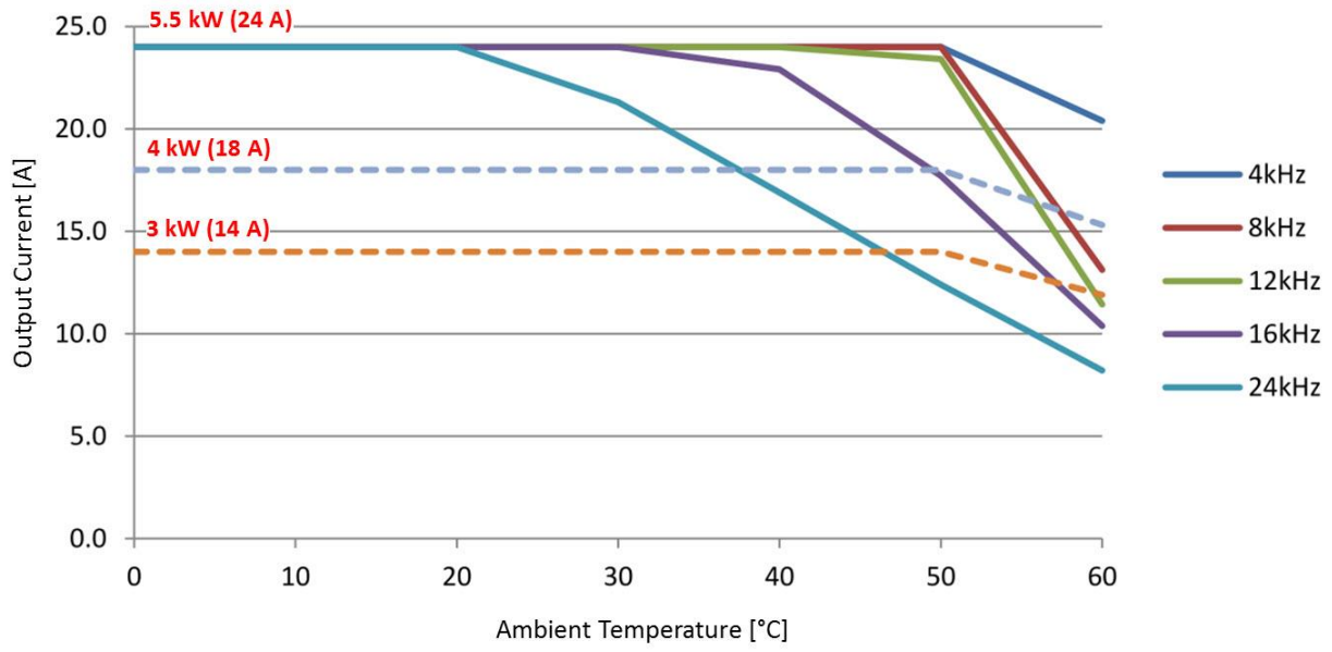
DC1, 230 V, Frame Size FS3, IP20
