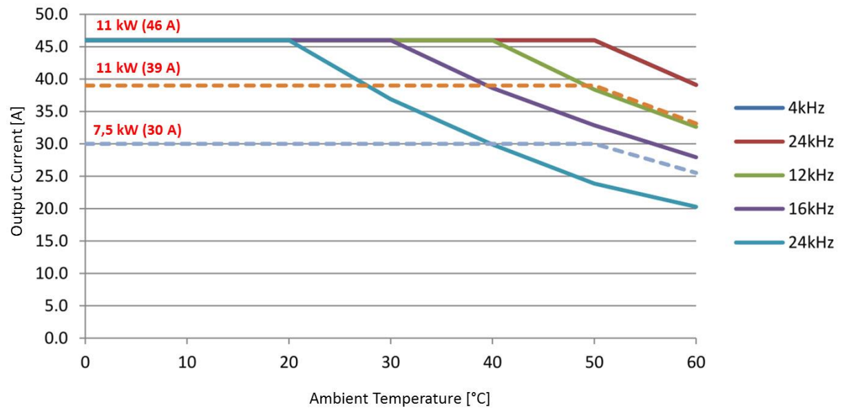
DC1...E1, 230 V, Frame Size FS4, IP20
