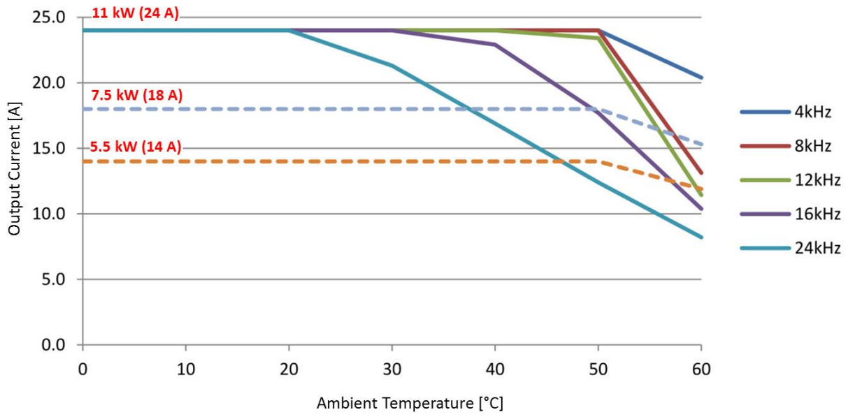
DC1...E1, 400 V, Frame Size FS3, IP20
