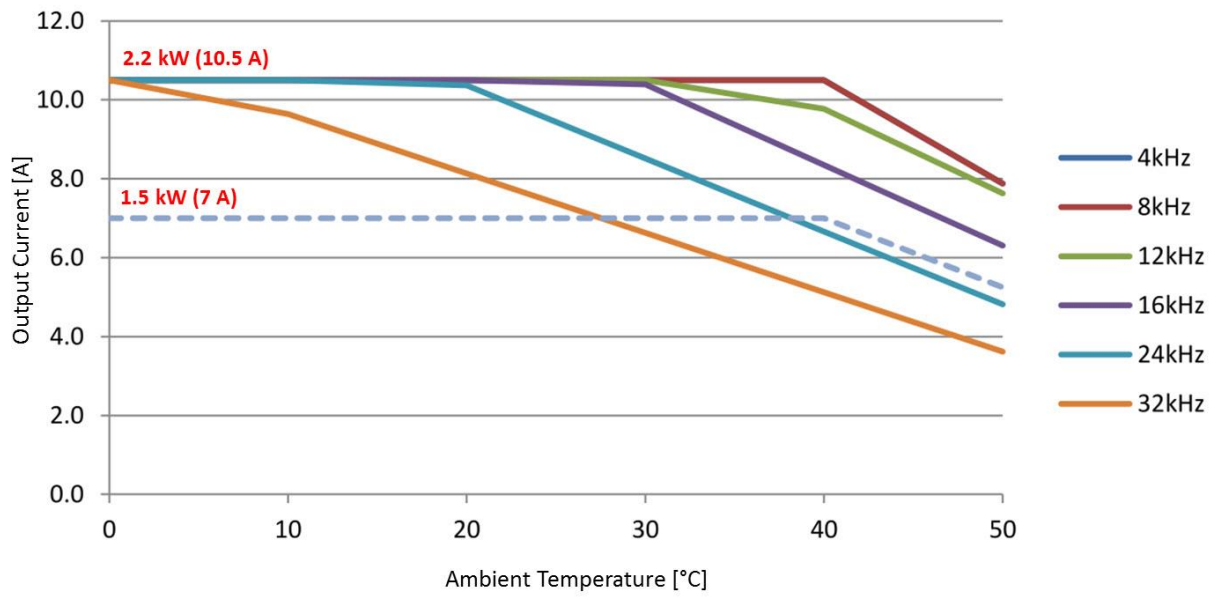
DC1...E1, 230 V, Frame Size FS2, IP66
