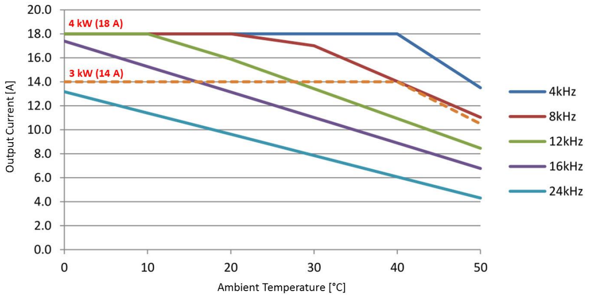
DC1...E1, 230 V, Frame Size FS3, IP66
