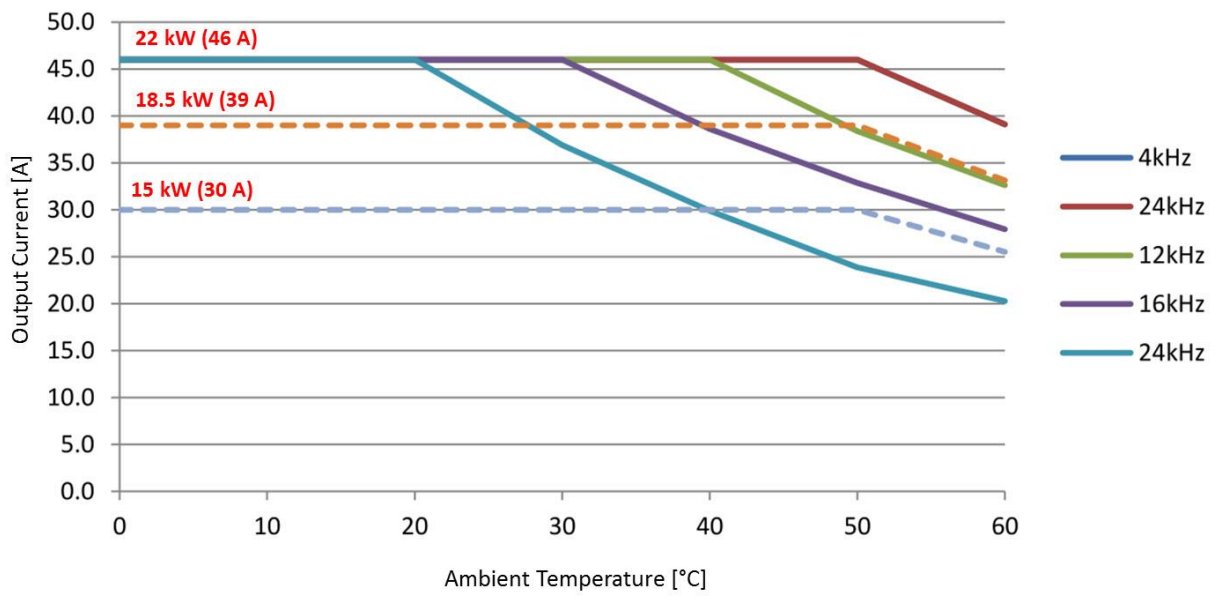
DC1...E1, 400 V, Frame Size FS4, IP20
