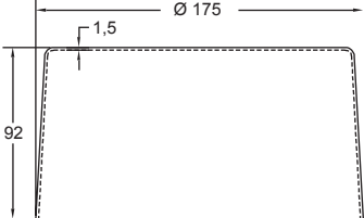
Aluminium kap
