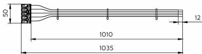
WT120Z TW-5x2.5-L1200
