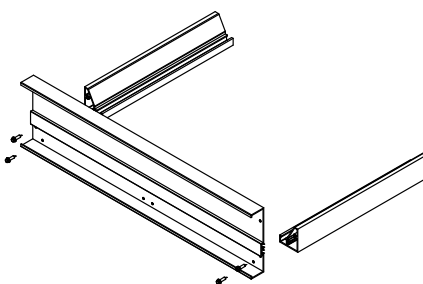
PSG33-0200 Shoulder profile
