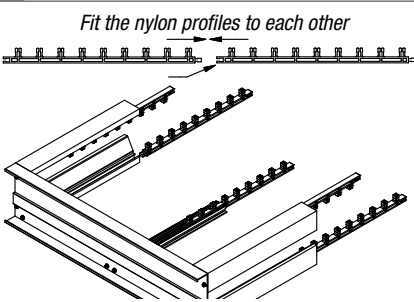
PSG33-0R03 Blade profile
