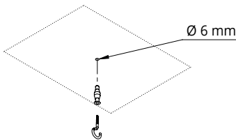
1 Fastening plasterboard
