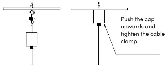
2 Mount and connect
