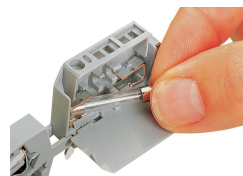
Fuse replacement: Easily removing a fuse by hand.
