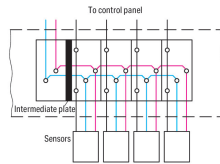
Power supply from control panel side
