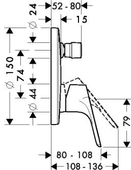
Focus 31946000
