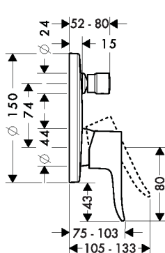
Logis 71407XX0
