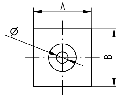
SKINTOP CUBE MODULE 20x20 / 40x40 (SMALL, LARGE, BLIND)
