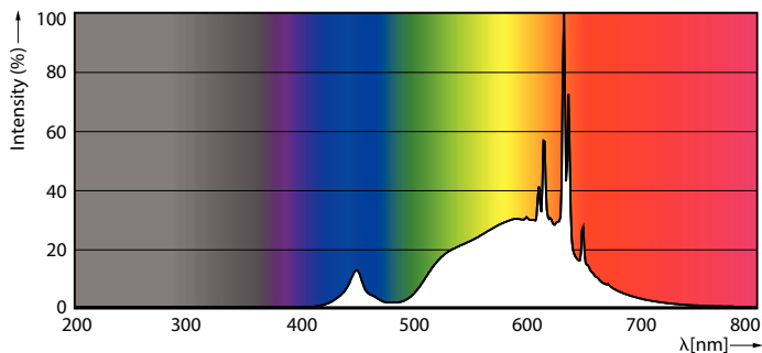
Spectral Power Distribution Colour - MAS LEDspot UE 2.1-50W GU10 ND 827
