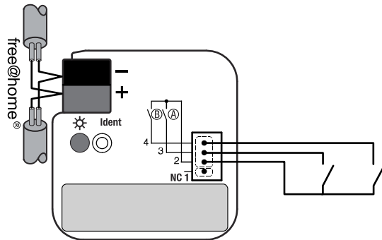
Fig. 4: Electrical connection 2-gang binary input, flush-mounted
