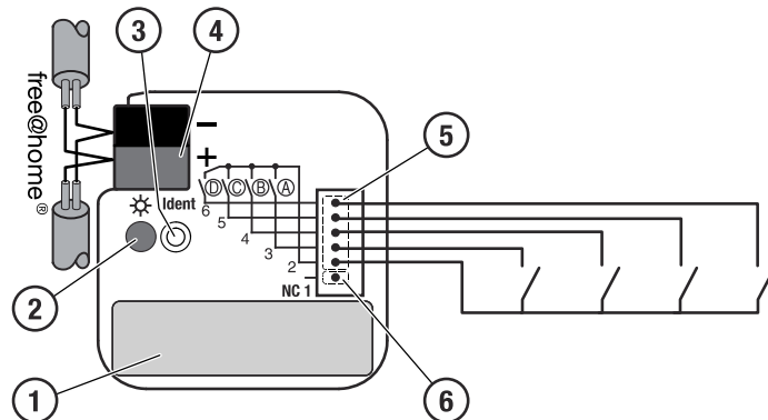
Fig. 2: Overview of devices 4-gang binary input, flush-mounted
