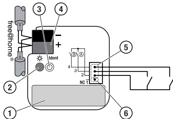
Fig. 1: Overview of devices 2-gang binary input, flush-mounted
