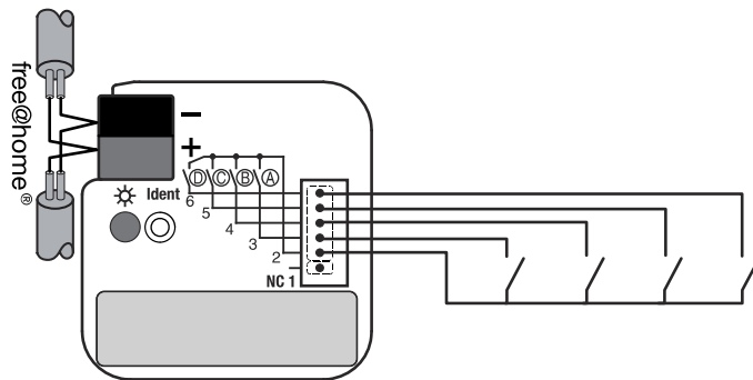
Fig. 5: Electrical connection 4-gang binary input, flush-mounted
