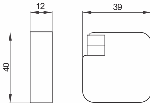
Fig. 3: Dimensions 2-gang binary input, flush-mounted/4-gang binary input, flush-mounted (specifications in mm)
