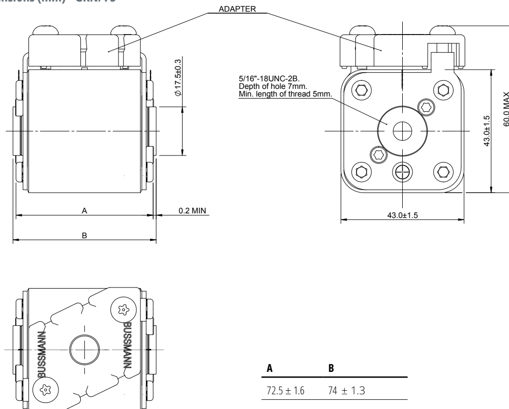
Dimensions (mm) - GKN/75
