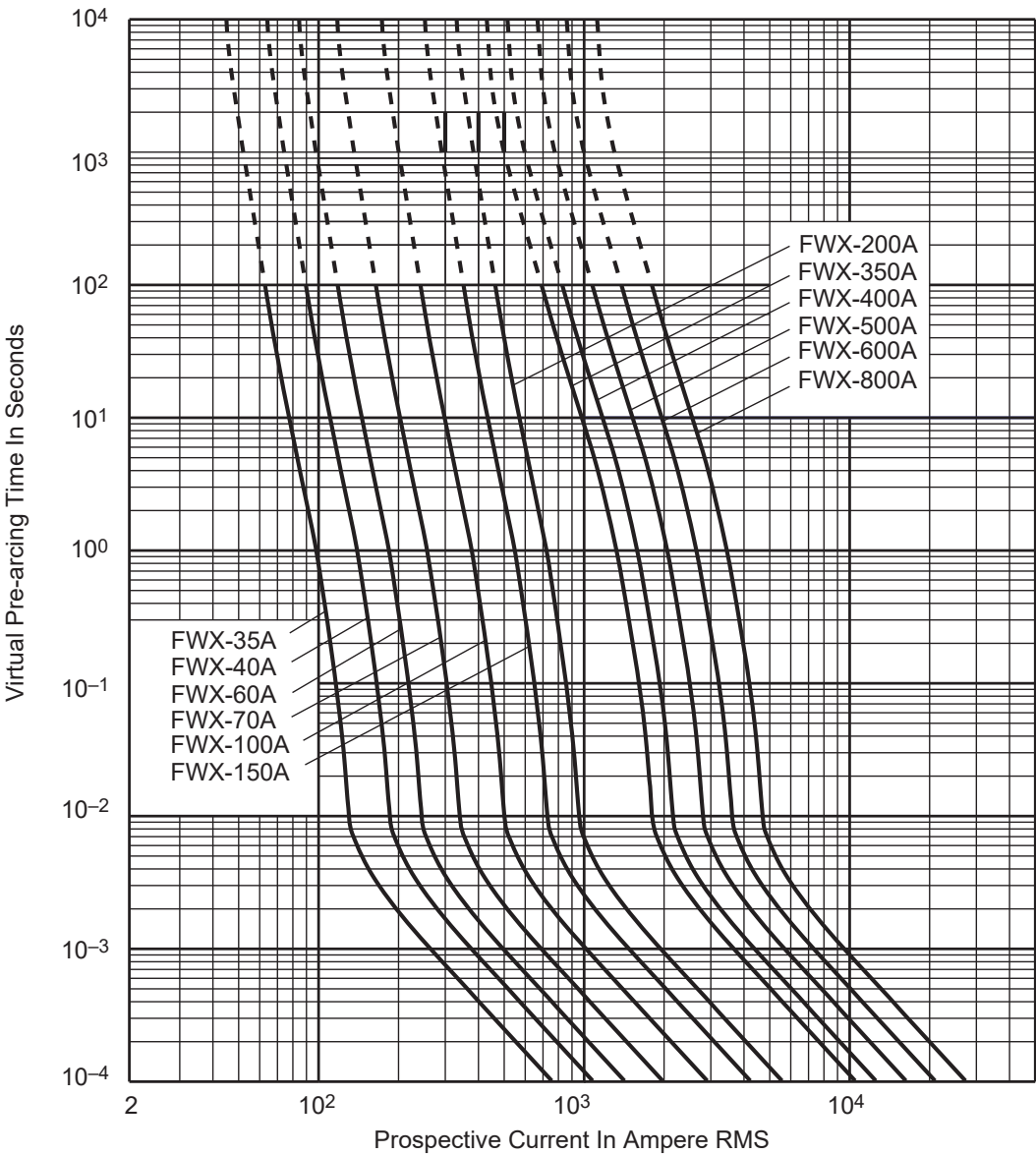
Time-current curve
