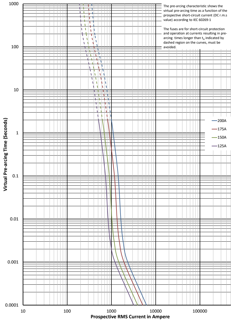
Time-current curve - 125 A to 200 A
