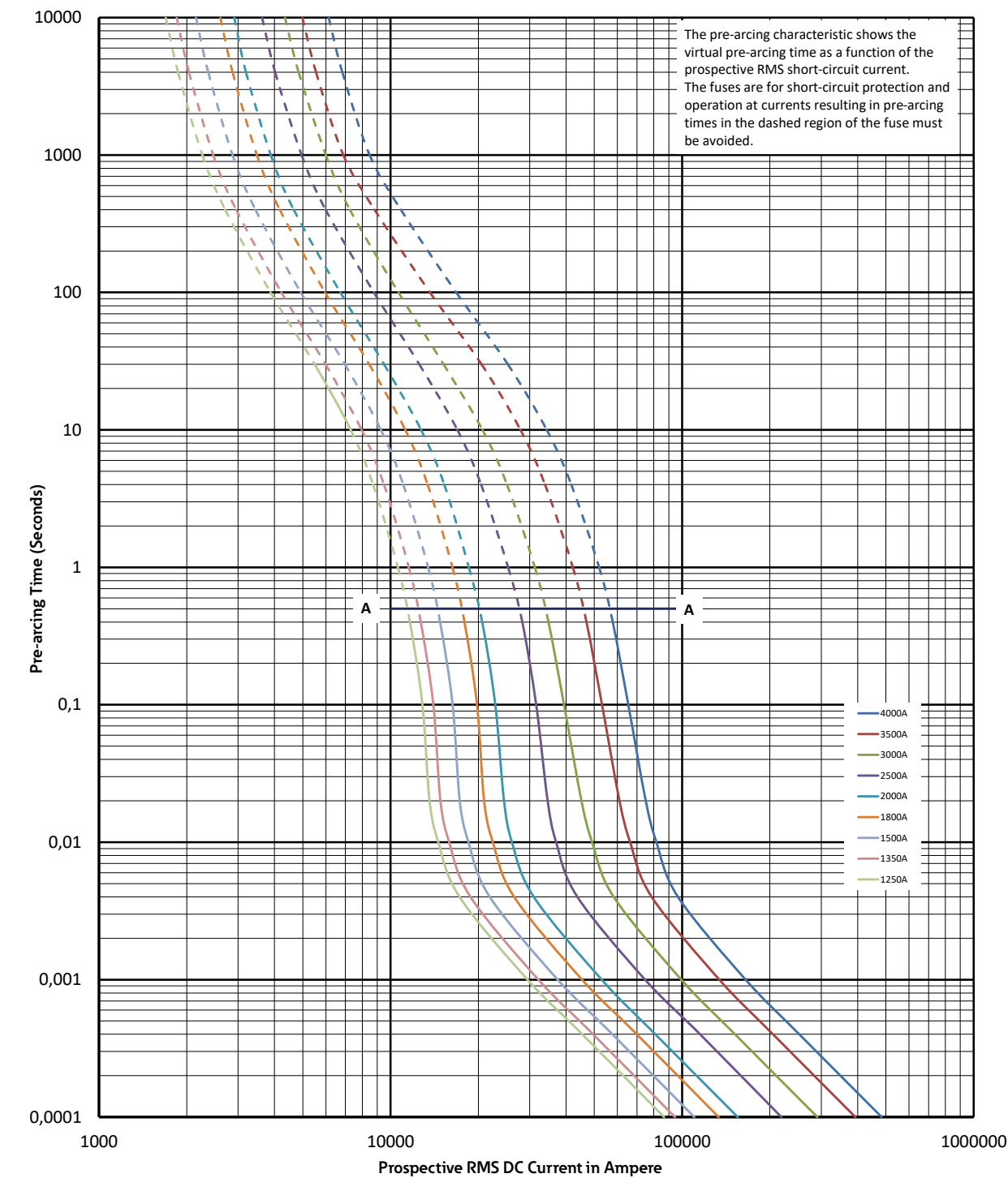
Time-current curve
