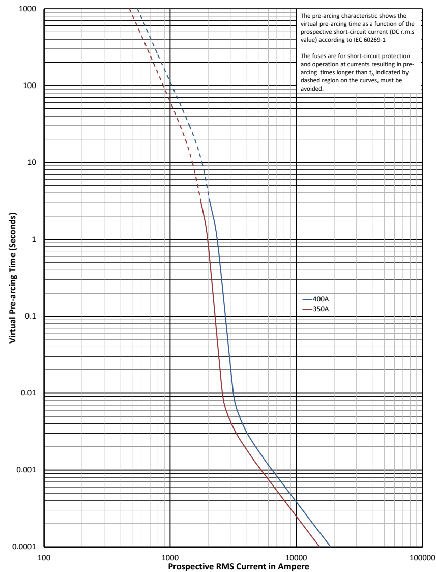
Time-current curve - 350 A and 400 A
