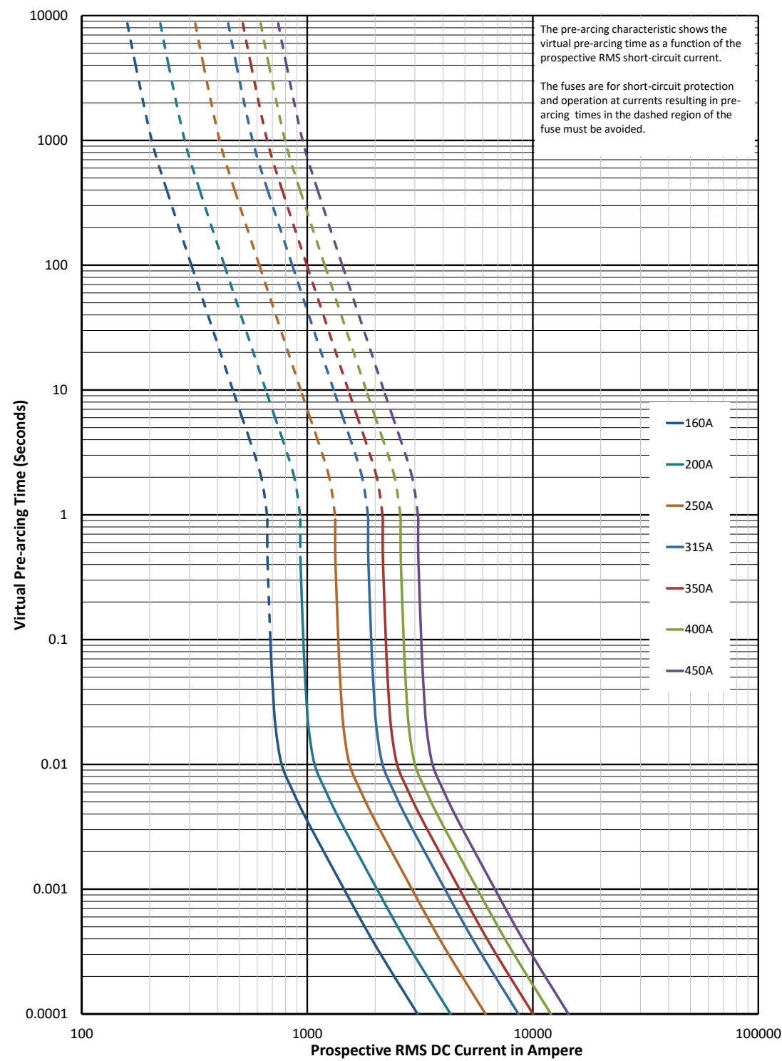
Time-current curve
