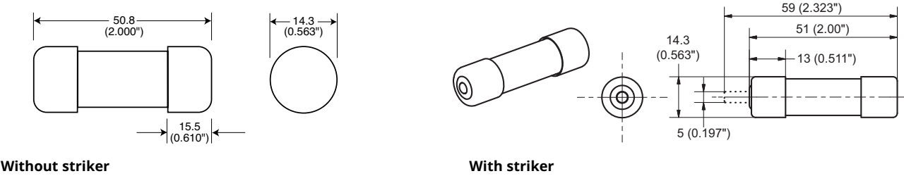
Dimensions - mm (in)
