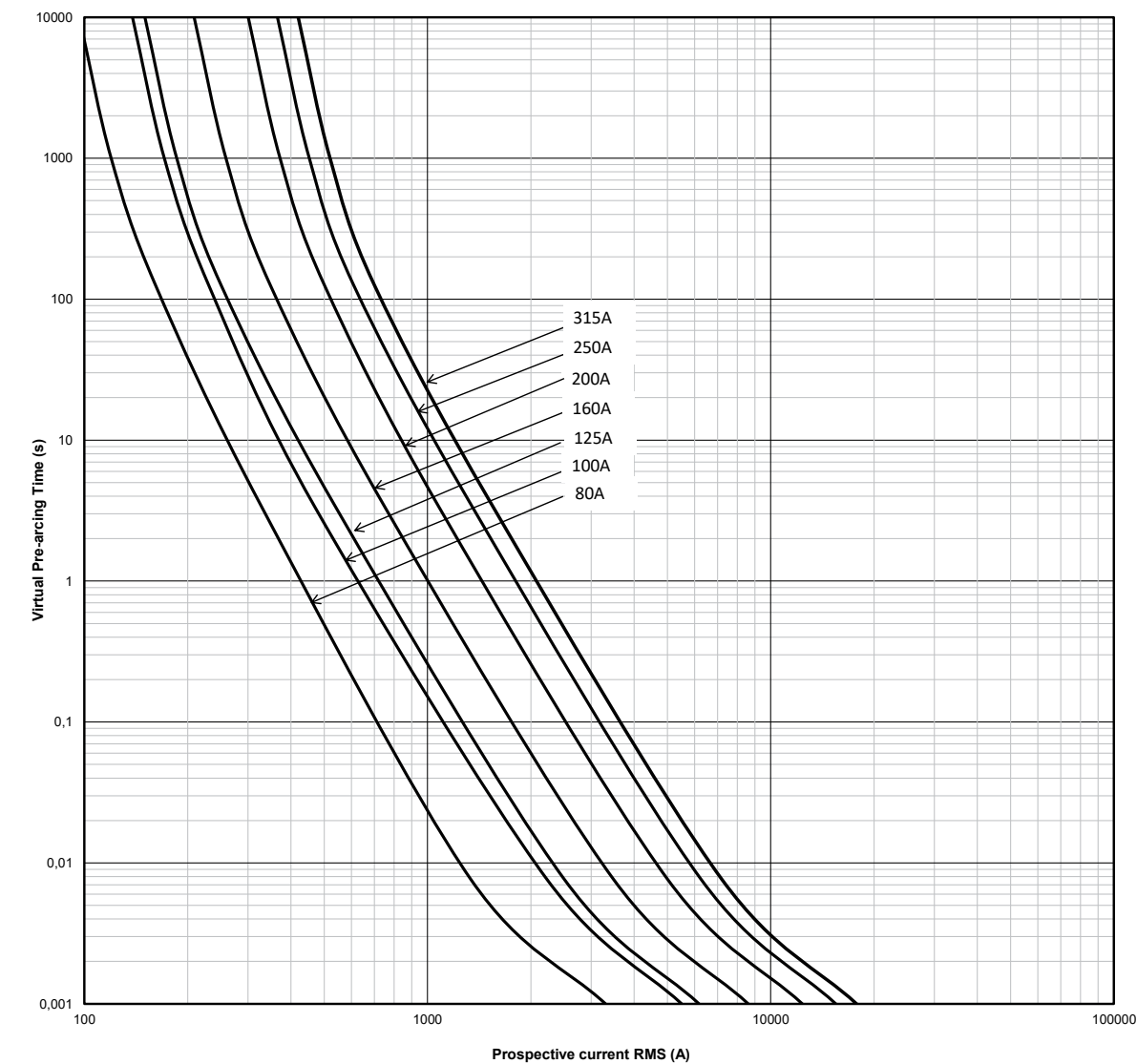
Time-current curve
