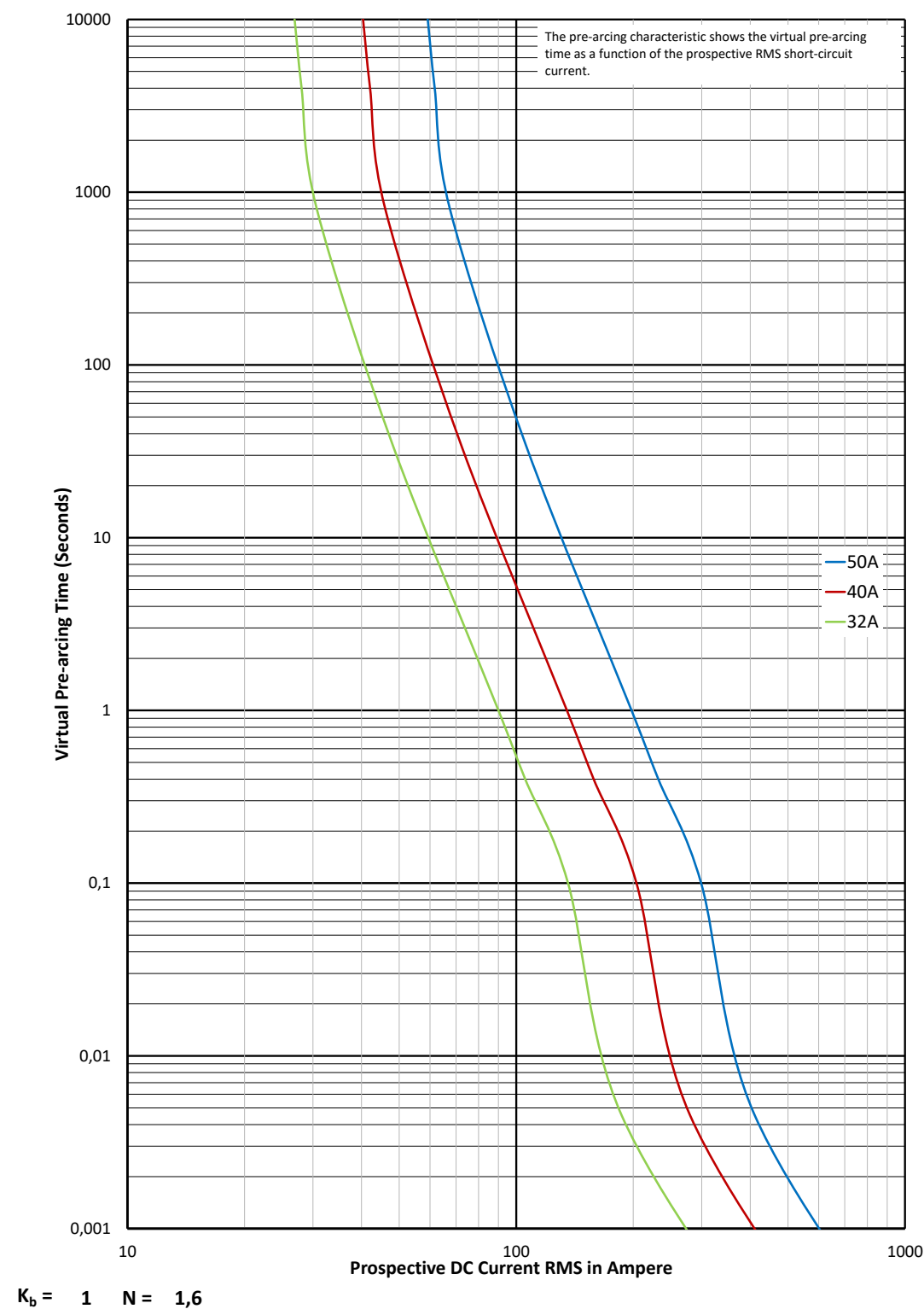
Time-current curve
