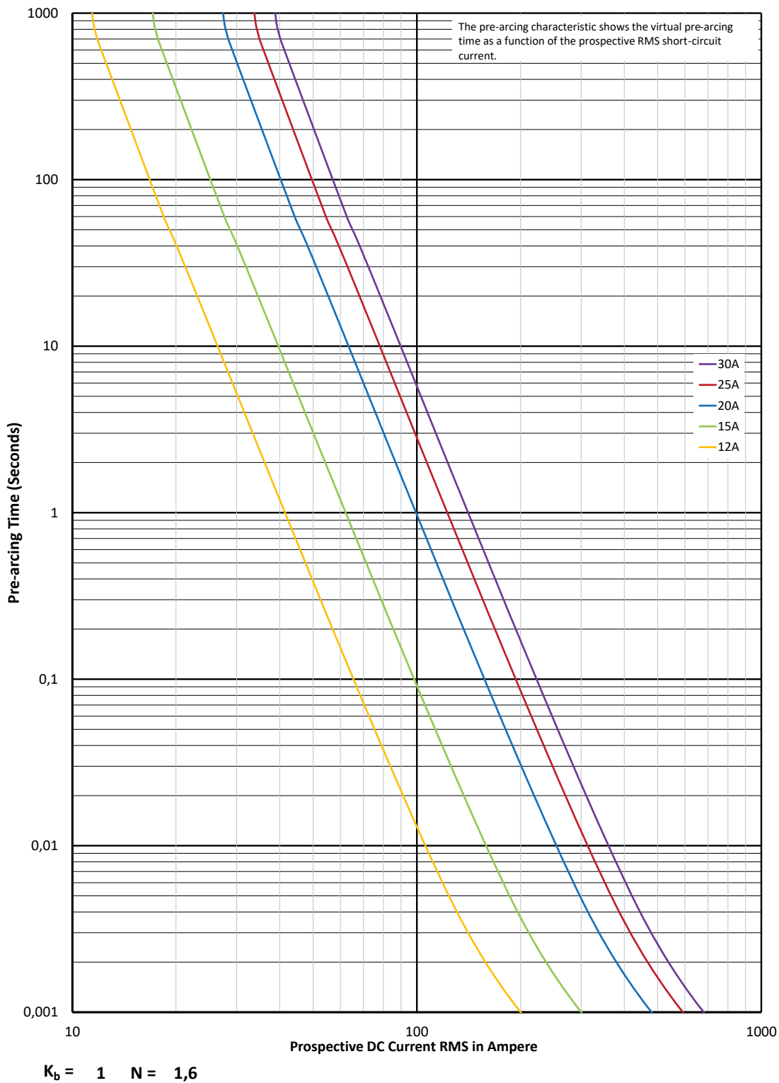
Time-current curve
