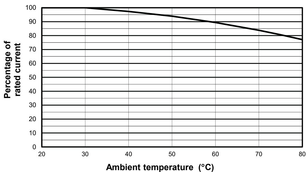
Temperature derating
