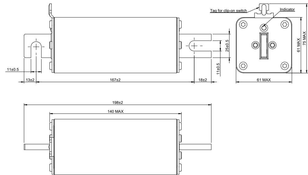
Dimensions (mm) - 2TN/170 (DIN)
