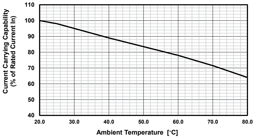
Temperature derating curve
