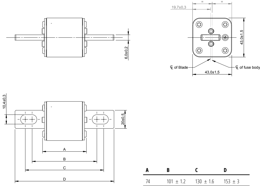
Dimensions (mm) - FU/115
