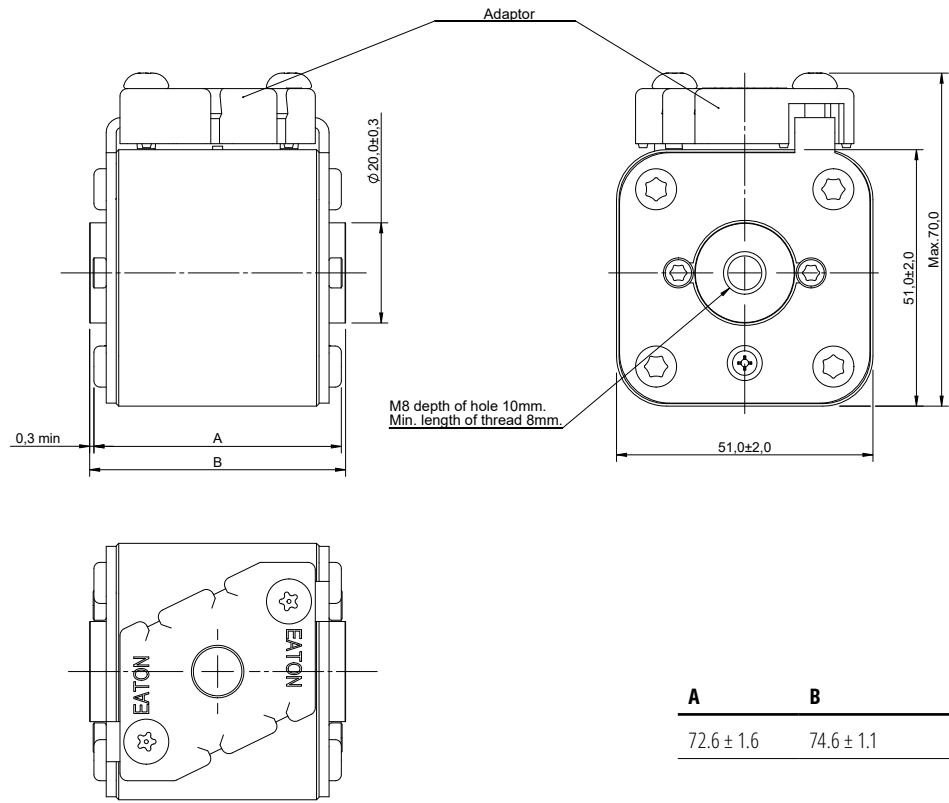
Dimensions (mm) - GKN/75
