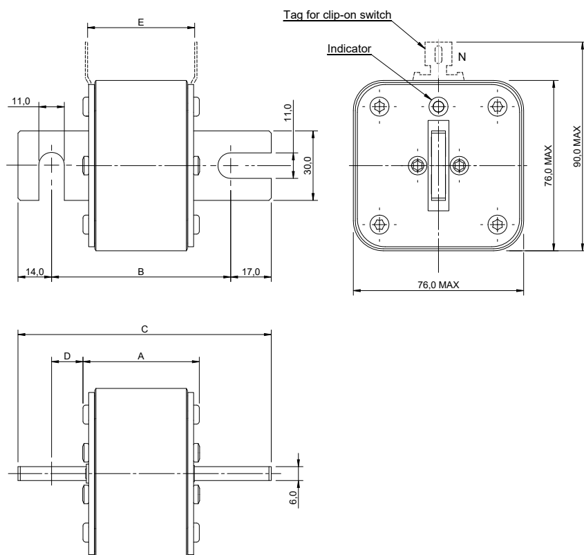
Dimensions (mm) - TN/110
