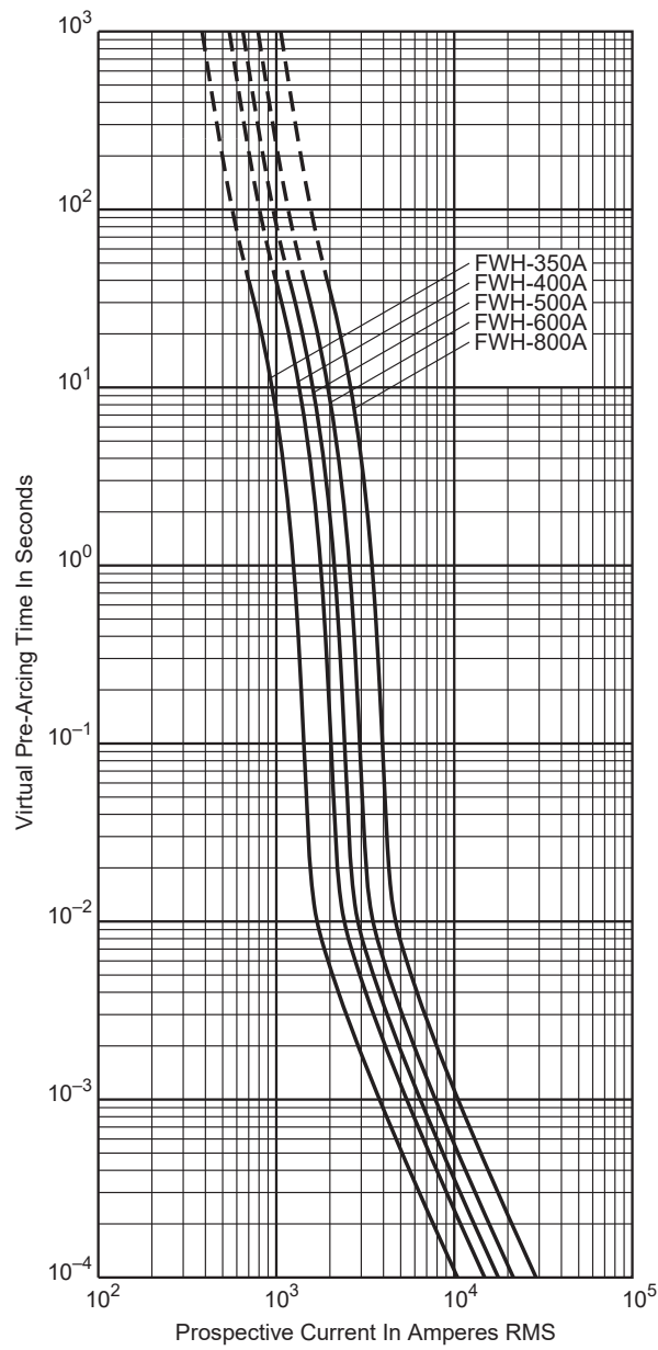
Time-current curve - 350 A to 800 A
