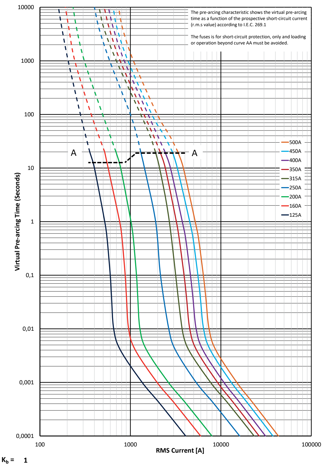
Time-current curve
