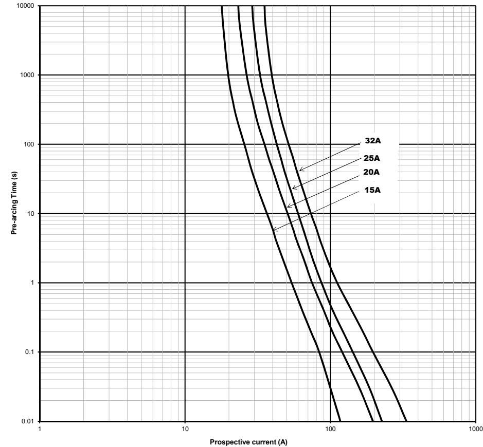
Time-current curve - 15 A to 32 A
