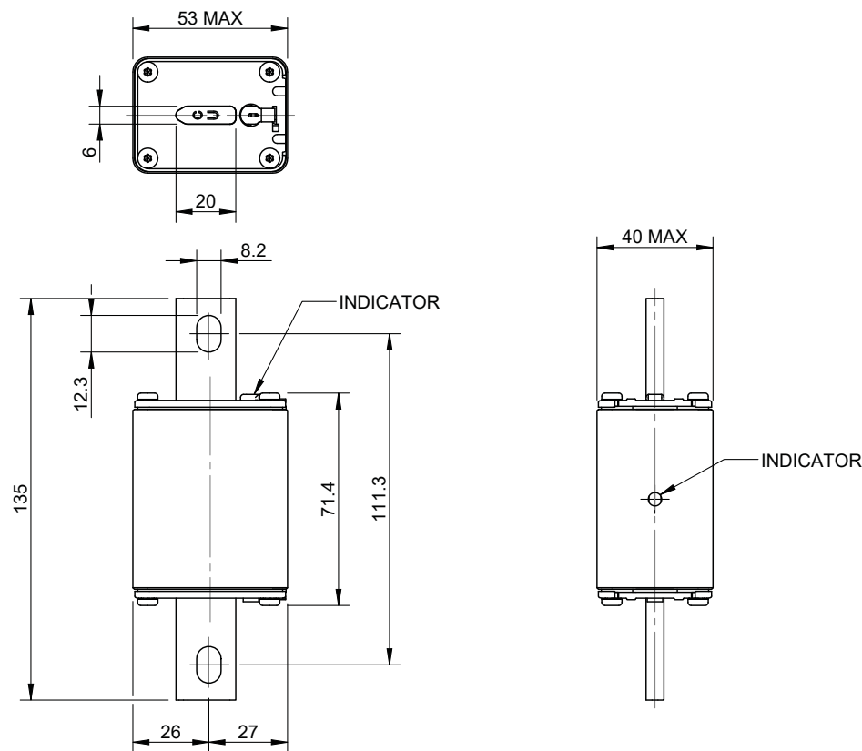
Dimensions (mm) - Size 1, bolted
