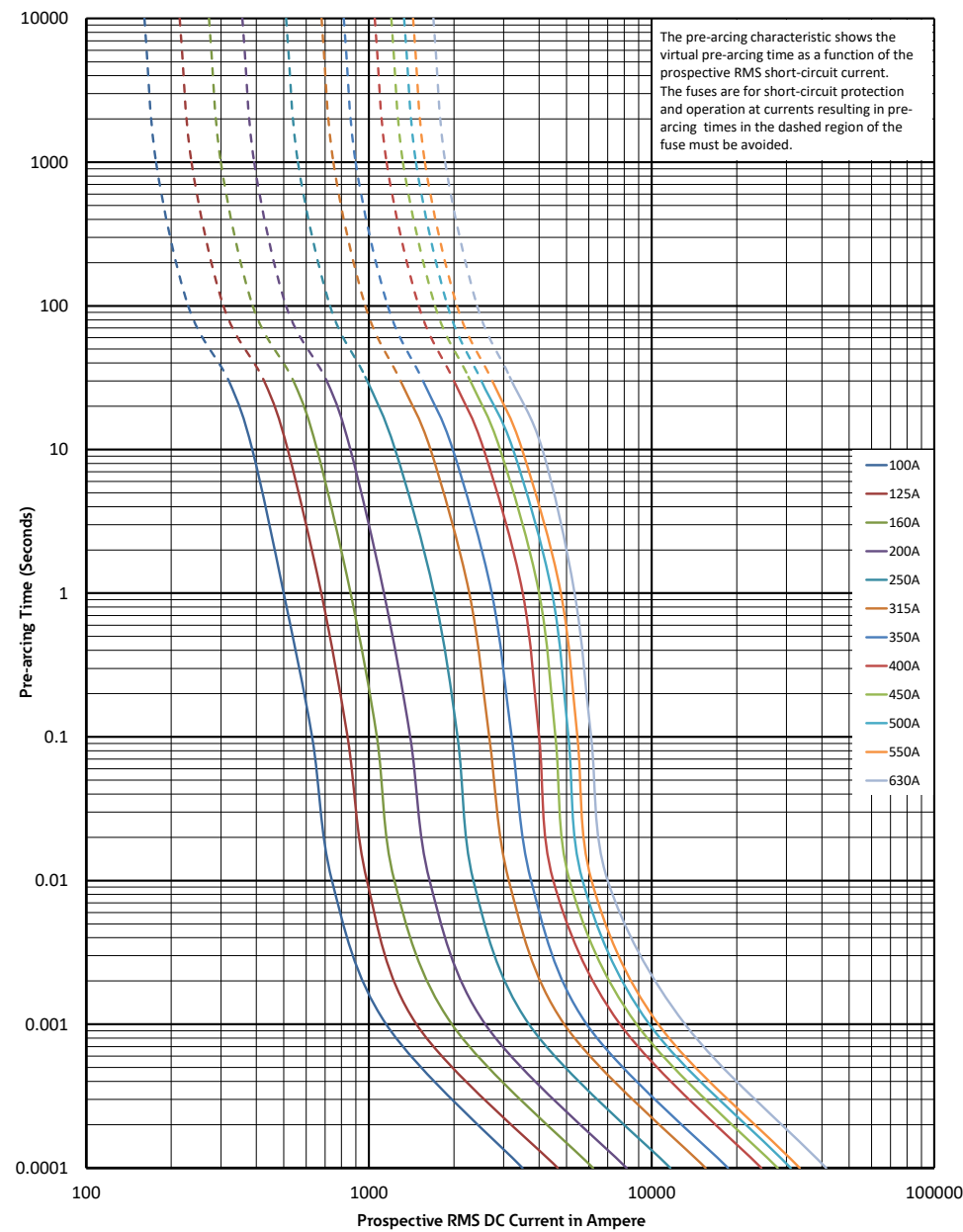
Time-current curve
