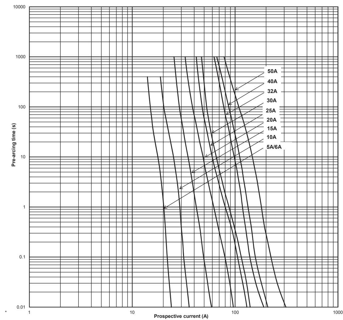
Time-current curve - 5 A to 50 A
