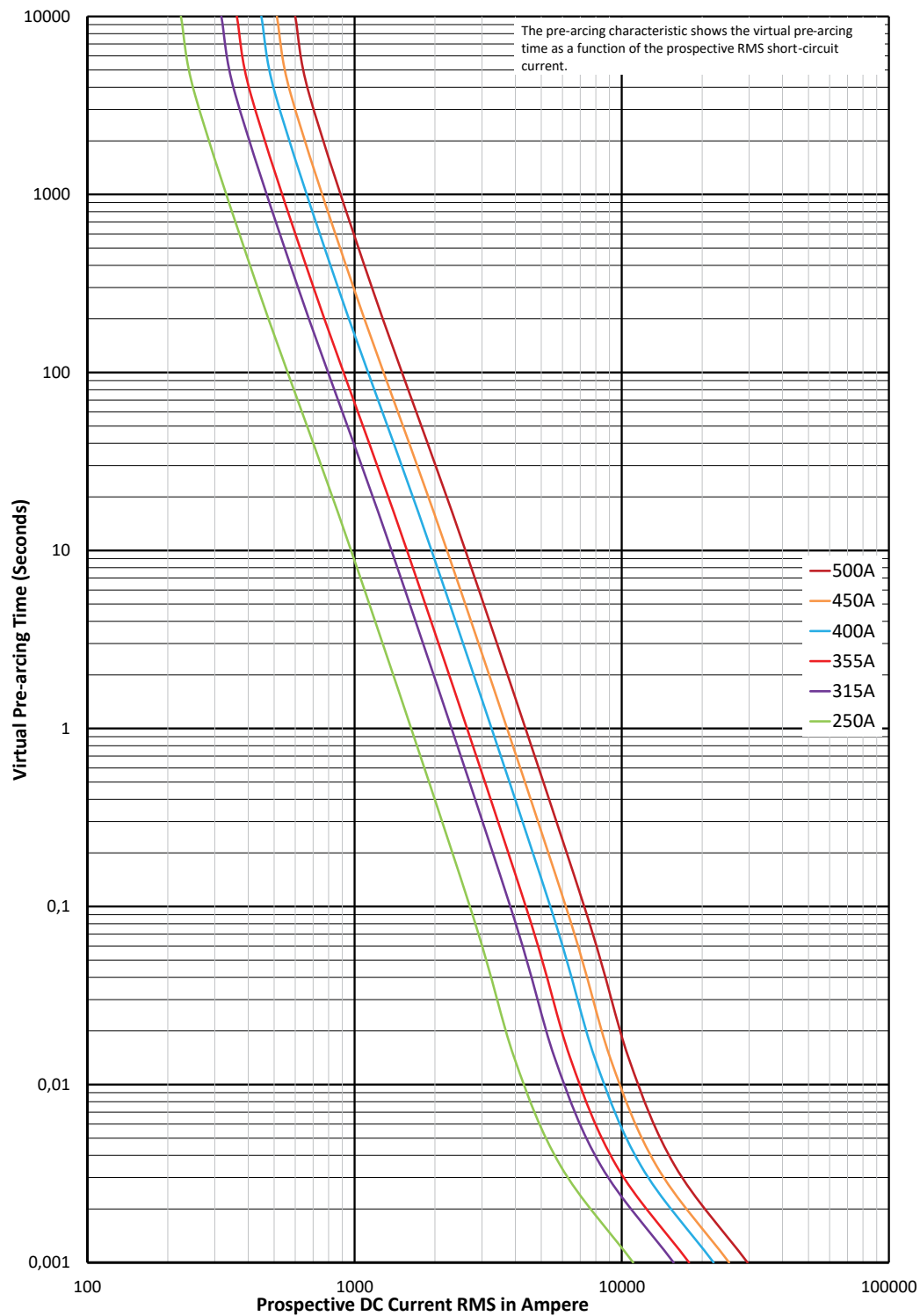
Time-current curve
