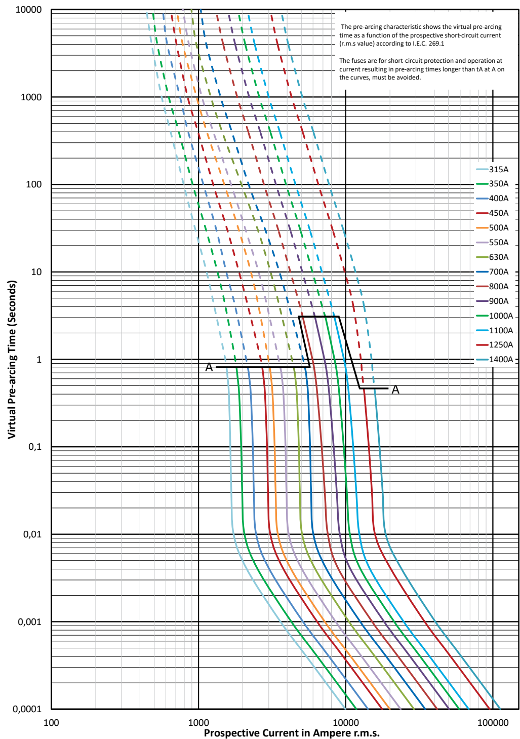
Time-current curve
