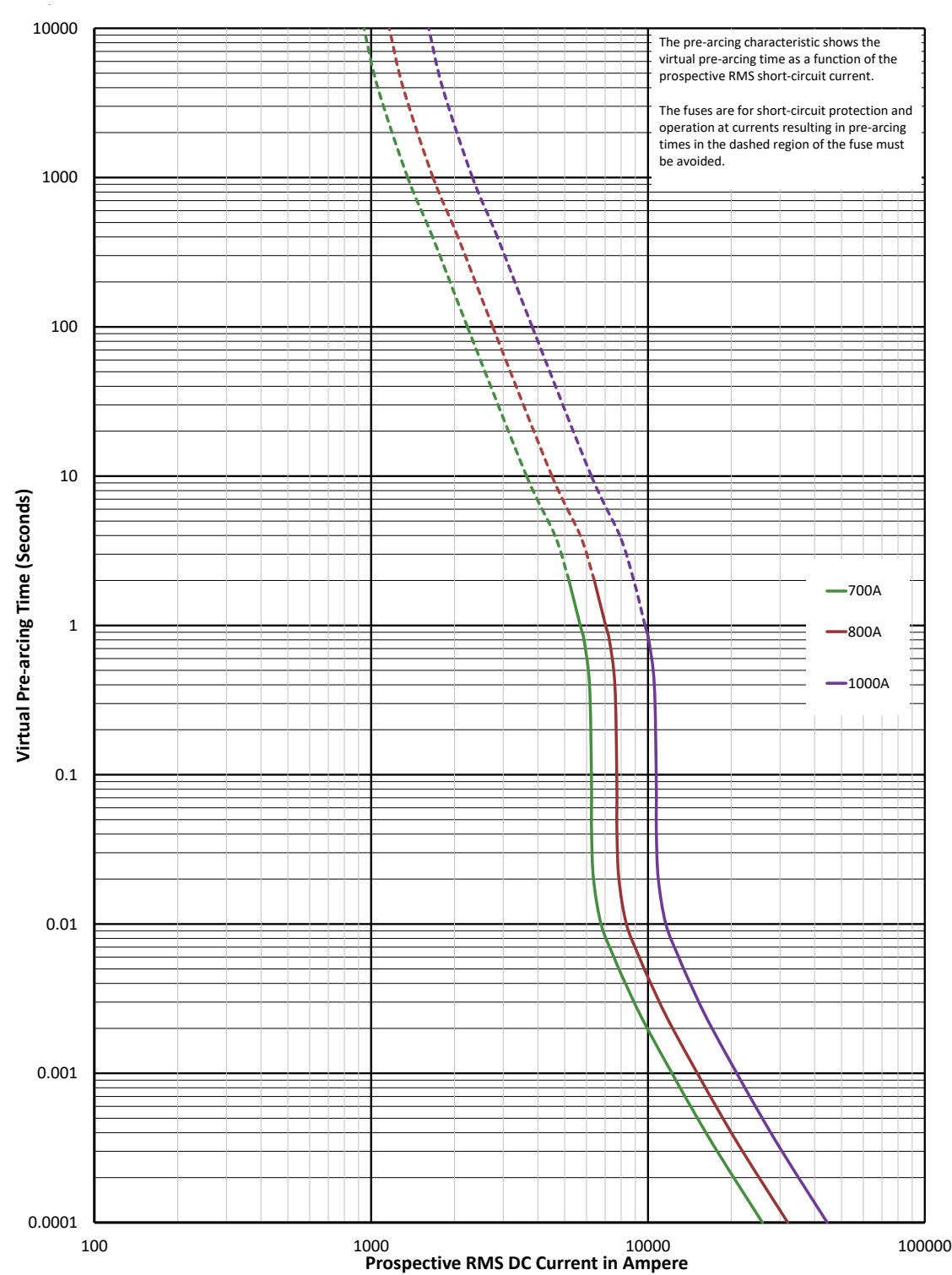
Time-current curve
