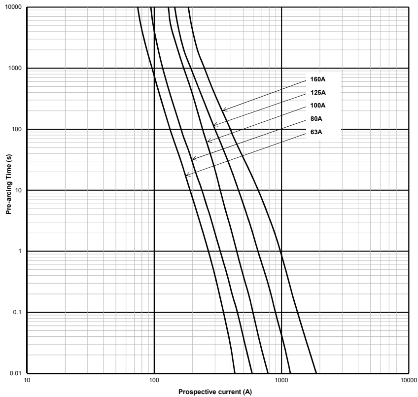
Time-current curve - Size 01XL, bladed and bolted, 1000 V d.c., 63 A to 160 A
