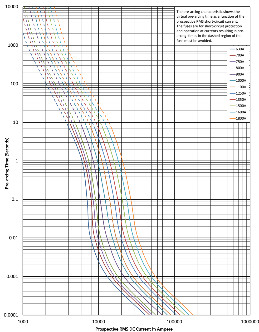
Time-current curve
