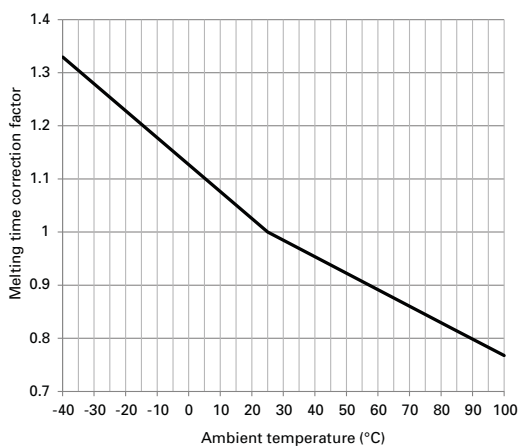
Temperature derating
