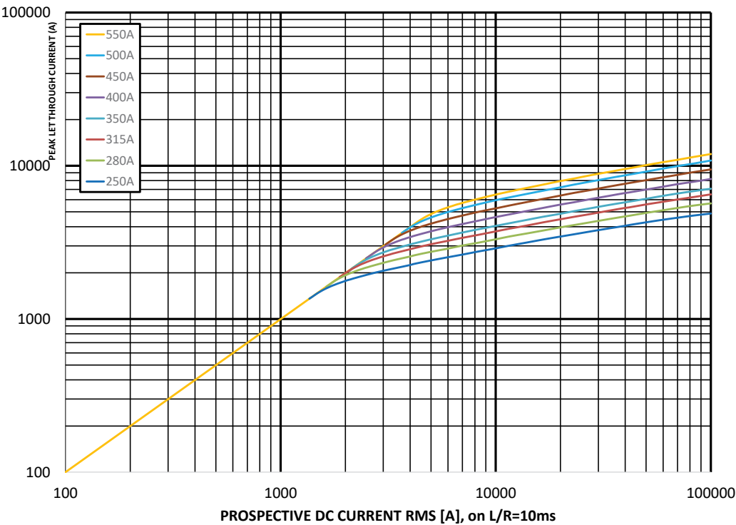
Peak let-through curve
