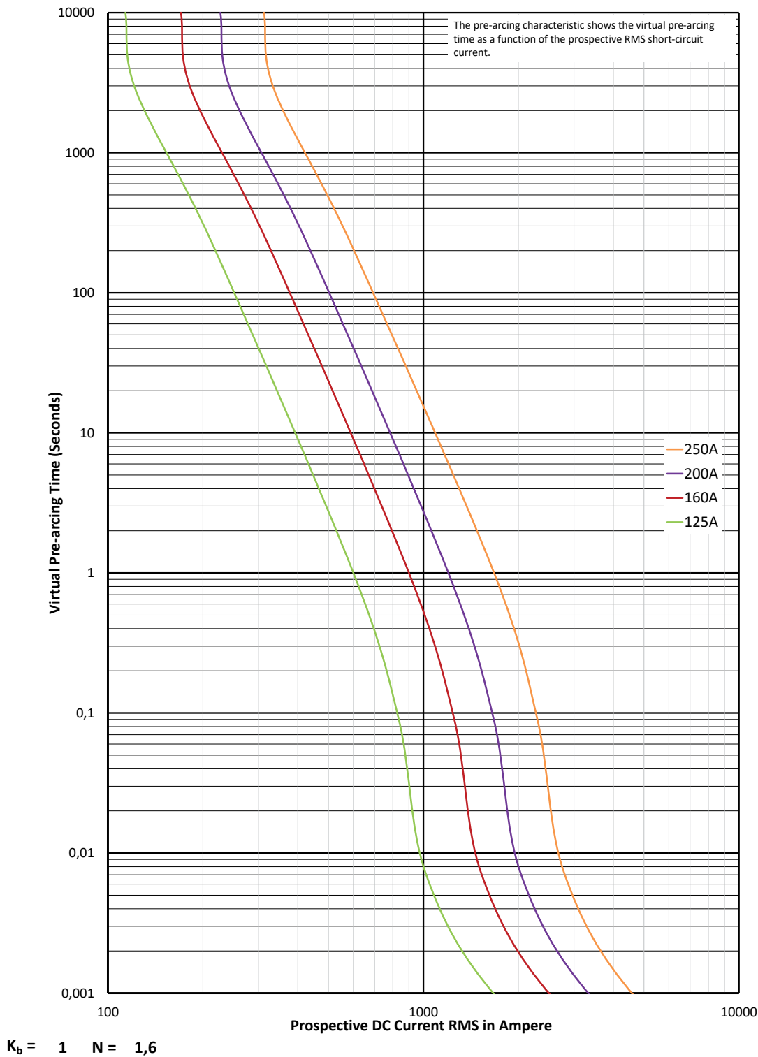
Time-current curve
