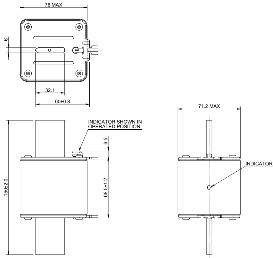
Dimensions (mm) - Size 3, bladed
