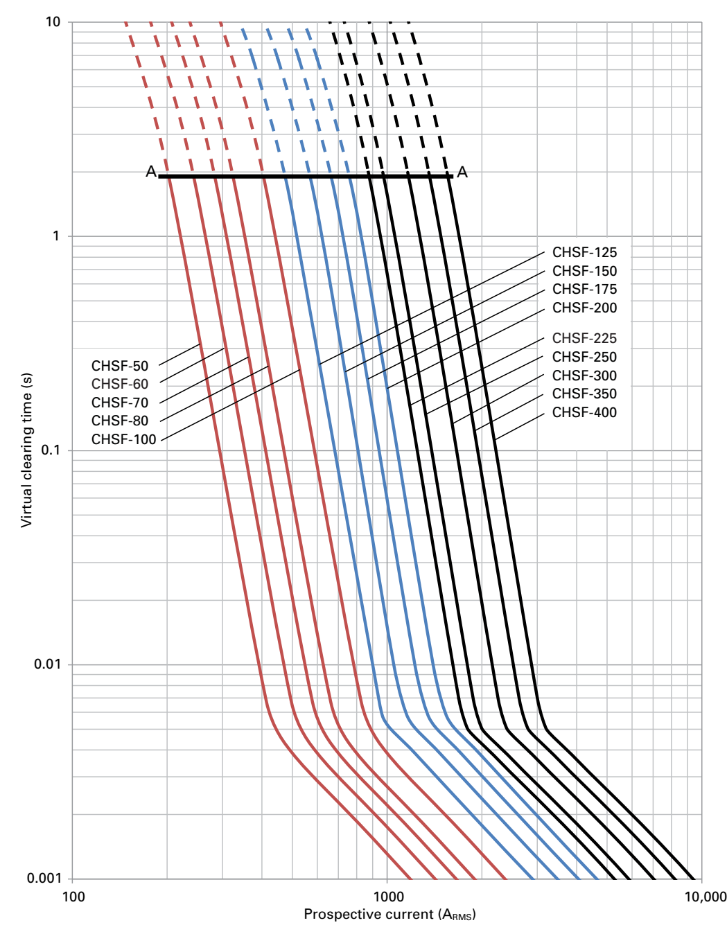
Time-current curve
