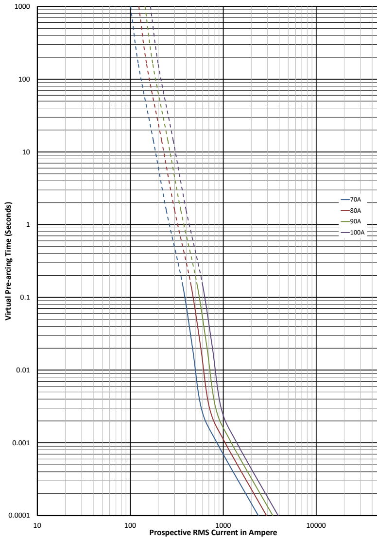
Time-current curve - 70 A to 100 A
