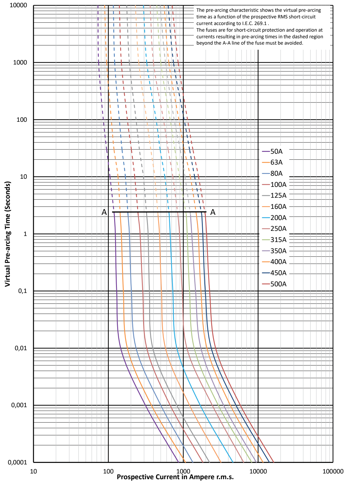
Time-current curve
