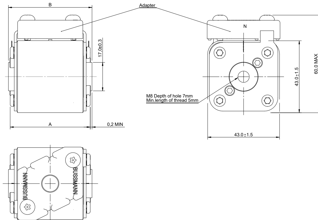
Dimensions (mm) - BKN/75
