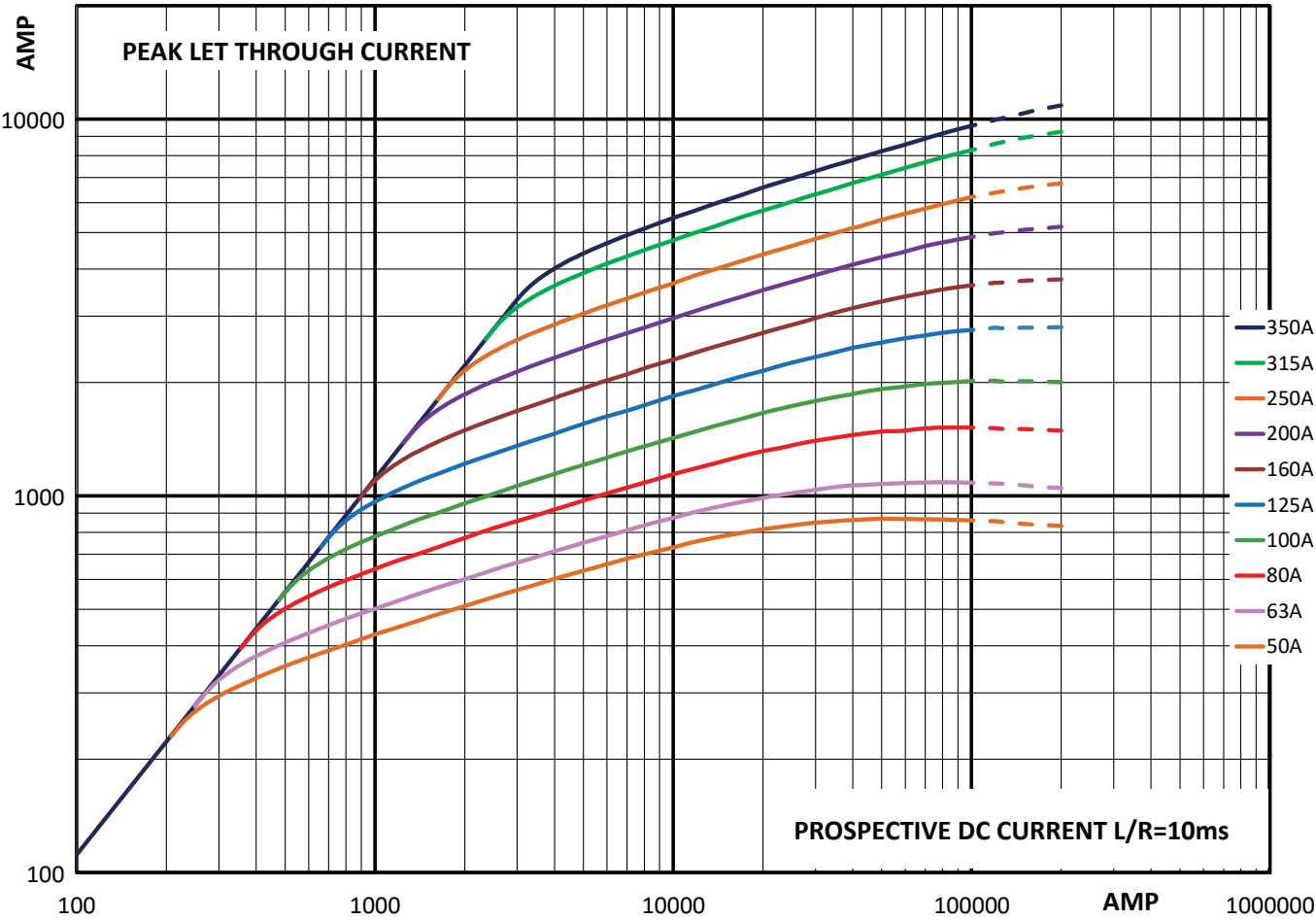
Peak let-through curve
