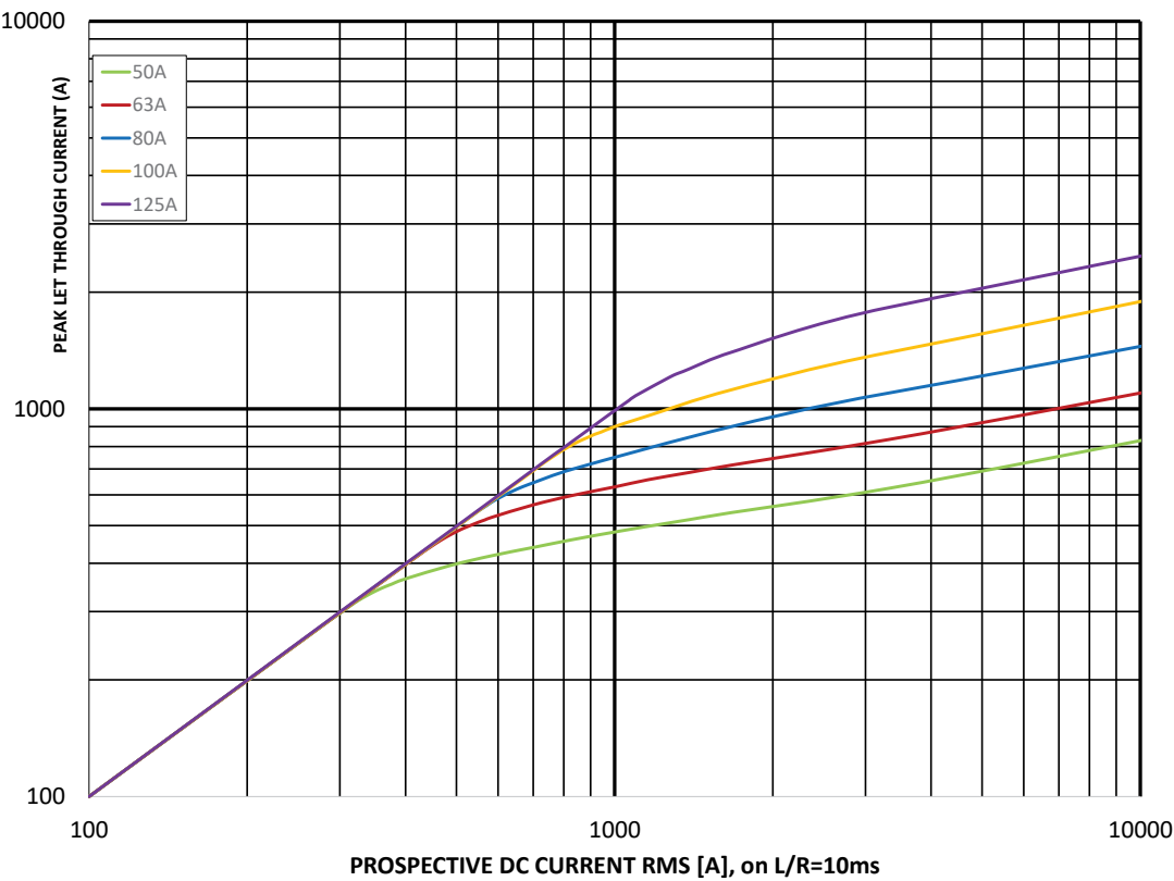
Peak let-through curve
