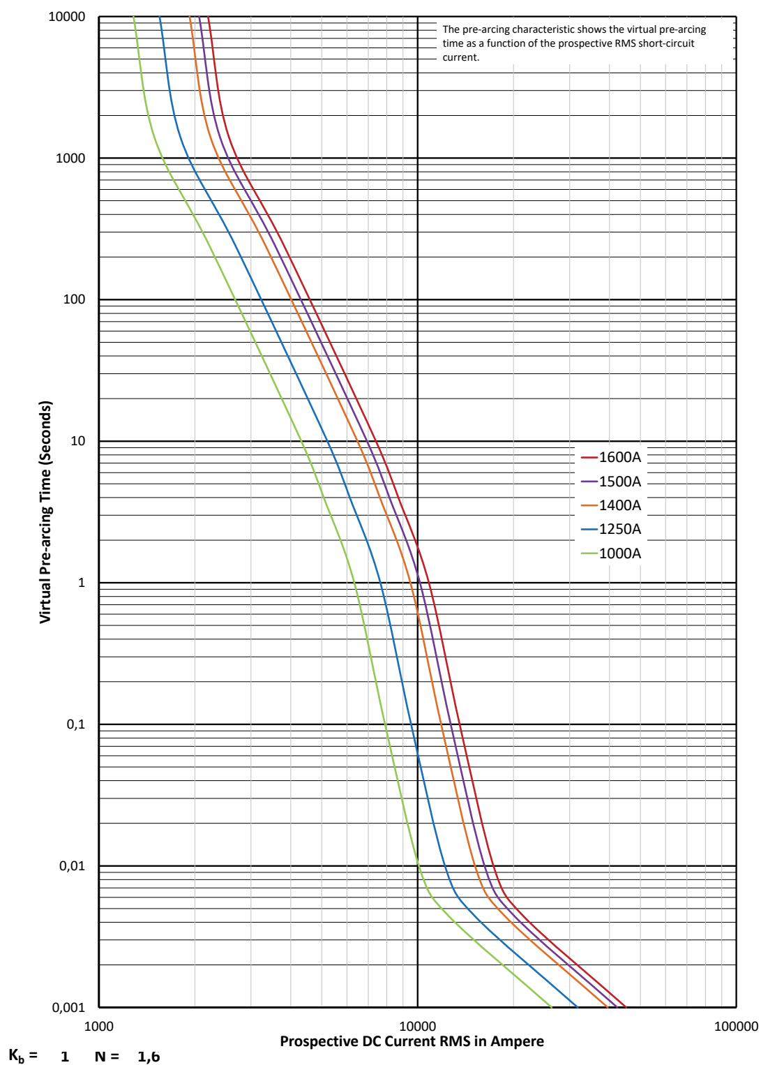
Time-current curve
