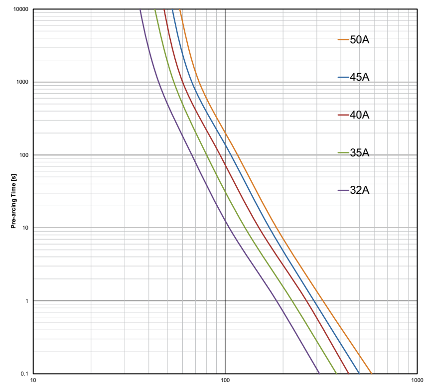
Time-current curve
