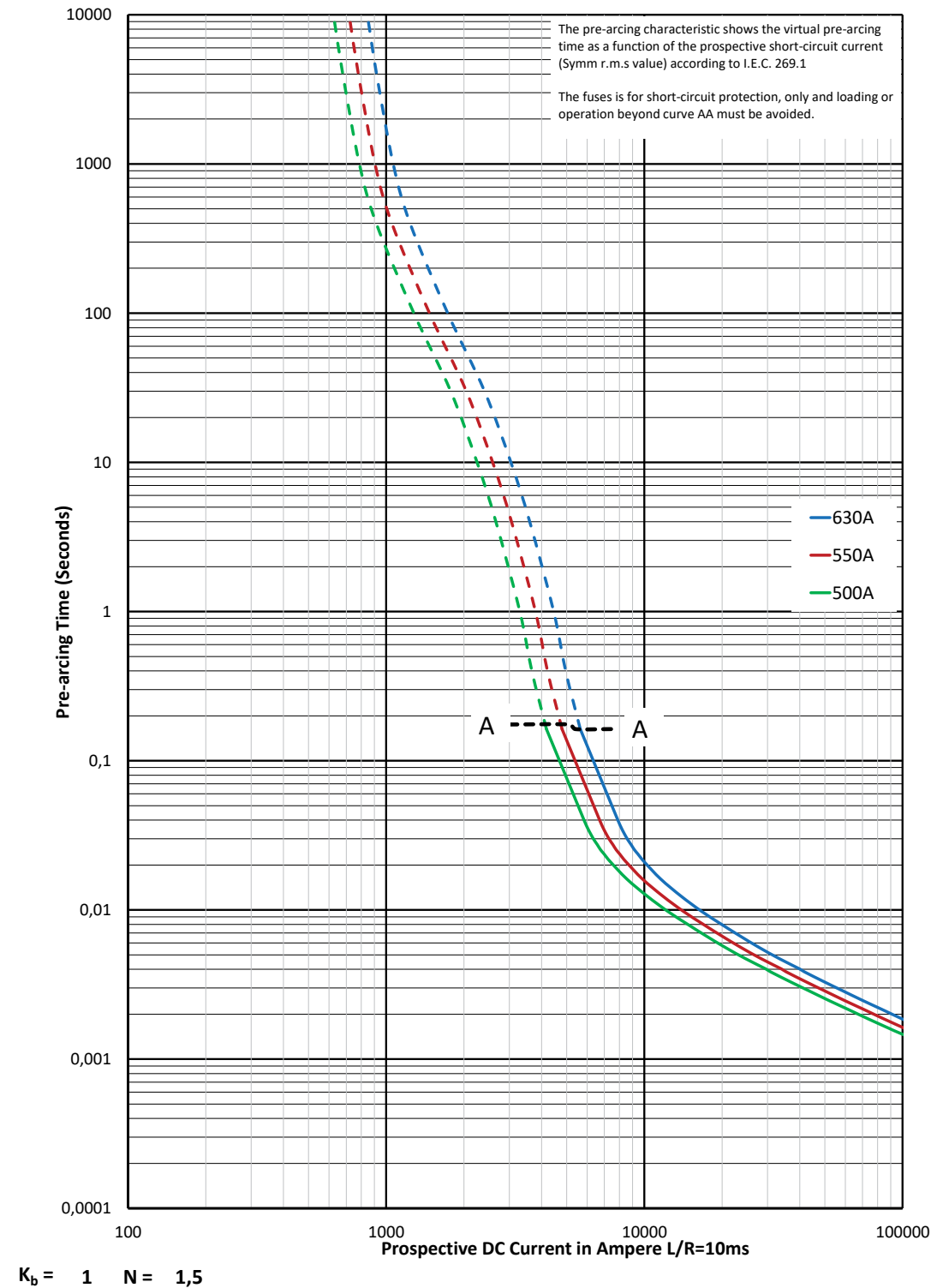
Time-current curve
