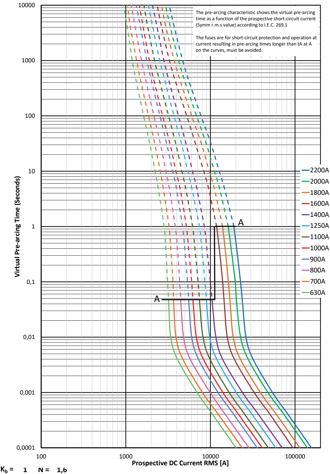
Time-current curve
