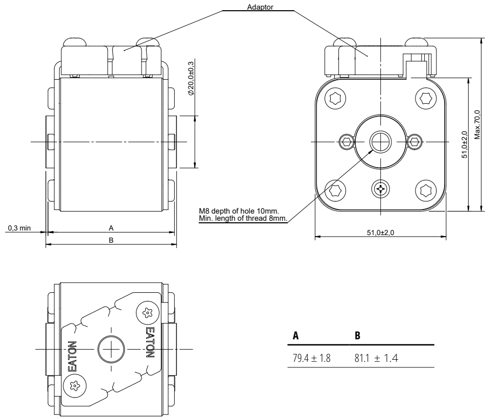
Dimensions (mm) - BKN/80
