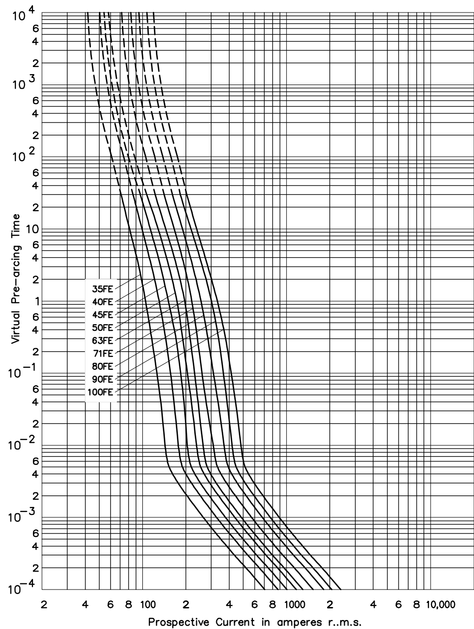
Time-current curve - FE, 35 A to 100 A
