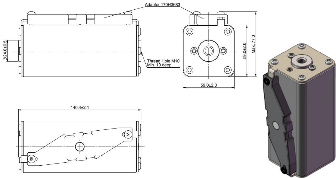
Dimensions (mm) - 2BKN/140 (Flush end)
