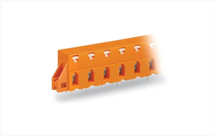
Color: ■ orange Similar to illustration Dimensions in mm L = (\text{pole no.} - 1) \times \text{pin spacing} + 6.5 \text{ mm} + 1.5 \text{ mm} L_1 = L + 5.8 \text{ mm} L_2 = L_1 + 6 \text{ mm}
