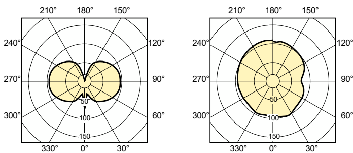
Light Distribution Diagram - MASTERC CDM-TC Elite 70W/930 G8.5 ICT/12
