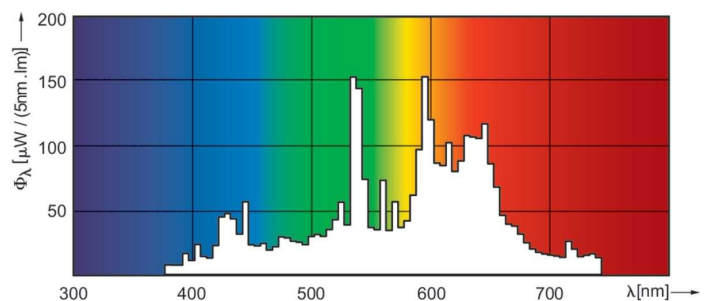
Spectral Power Distribution Colour - MASTERC CDM-TC Elite 70W/930 G8.5 ICT/12
