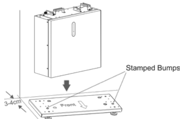
Step 2: Placing the Battery on the Bottom support
