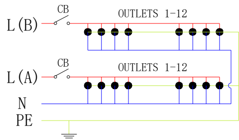
CIRCUIT SCHEMATIC
