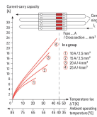
Application Notes on Terminal Blocks for Glass Cartridge Fuses Diagram: "Block Arrangement"
