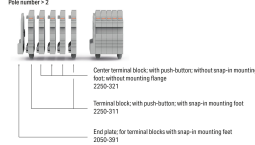
Example of a 5-pole terminal strip; with push-buttons; with snap-in mounting foot
