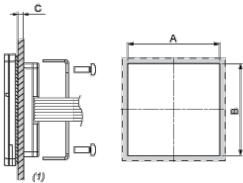
(1) Installation panel
