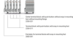
Example of a 5-pole terminal strip; with push-buttons; with snap-in mounting foot Pole number > 2
