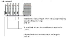
Example of a 5-pole terminal strip, with push-buttons, with snap-in mounting foot Pole number = 2
