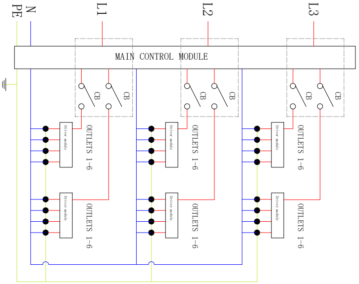
CIRCUIT SCHEMATIC
