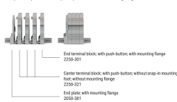
Example of a 4-pole terminal strip, with push-buttons, with mounting flange
