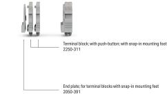
Example of a 2-pole terminal strip; with push-buttons; with snap-in mounting feet
