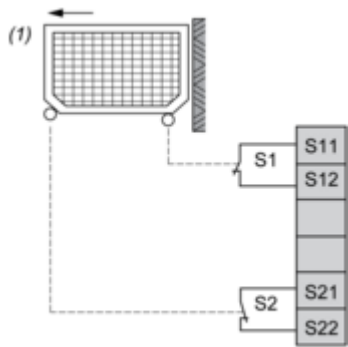
(1) Protective guard
