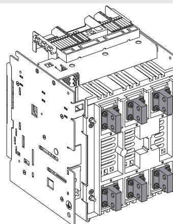
Figure 53 - W - VR - Arrière verticales IEC
