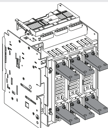
Figure 60 - W - HR - Arrière horizontales UL Listed
