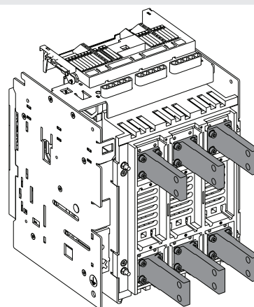
Figure 61 - W - VR - Arrière verticales UL Listed
