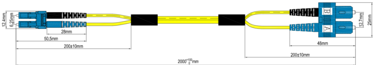
Dimensional drawing
