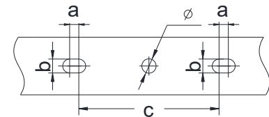
Mounting hole
