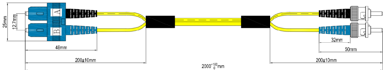
Dimensional drawing
