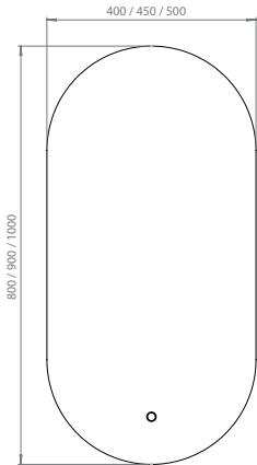
A-Line Oval
