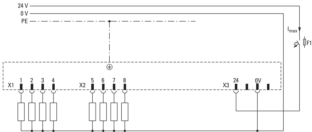
Figure 59: Wiring example
