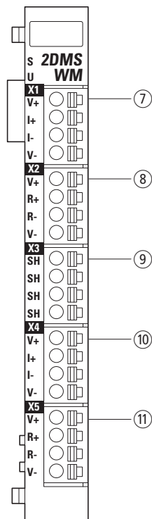
Figure 137: Pin assignment
