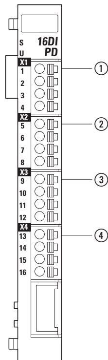
Figure 29: Pin assignment
