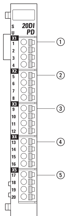
Figure 32: Pin assignment
