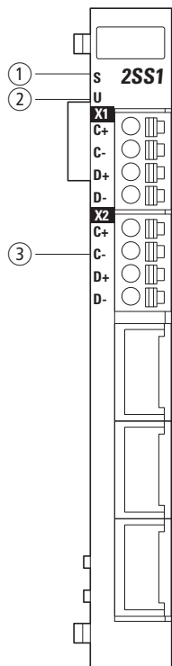
Figure 163: XN-322-2SSI LEDs
