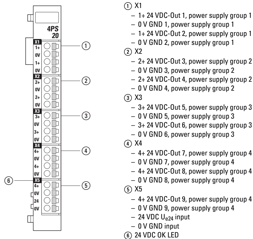
Figure 17: LED signals and pin assignment for XN-322-4PS-20
