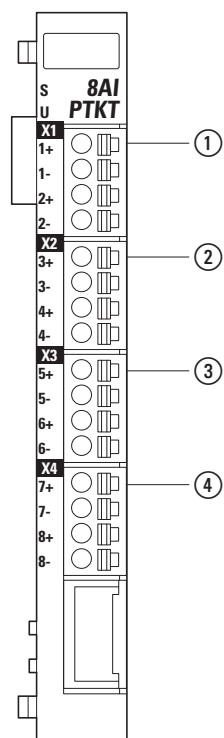
Figure 102: Pin assignment
