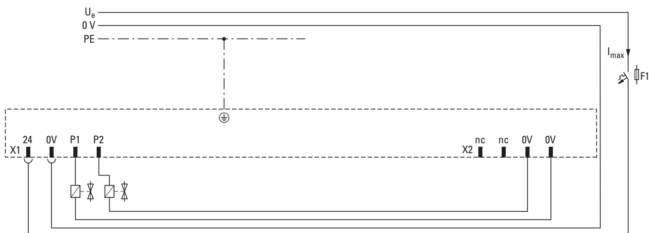
Figure 171: Wiring diagram with wiring for P1 and P2
