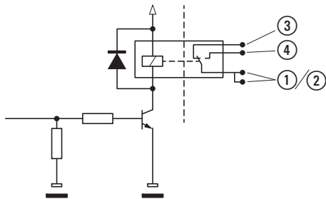
Figure 54: Internal logic for relay output
