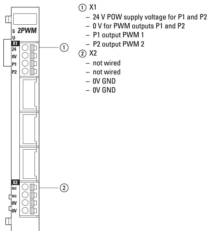
Figure 170: Pin assignment
