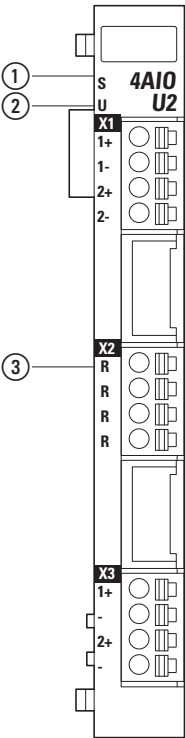
Figure 116: LED signals and pin assignment
