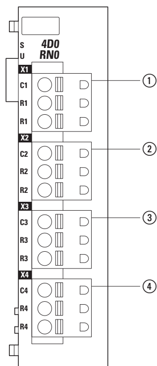
Figure 47: Pin assignment
