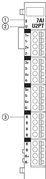
Figure 93: LED signals and pin assignment
