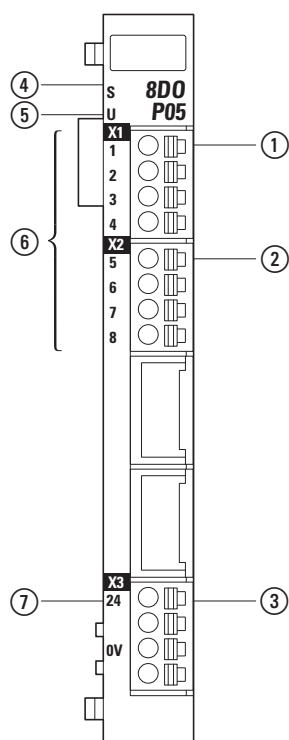
Figure 58: Pin assignment and status LED signals
