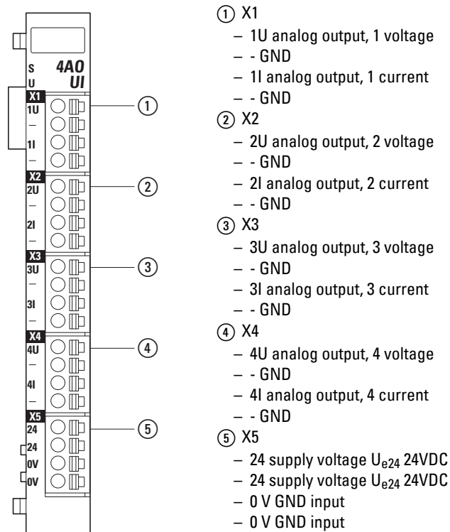
Figure 109: Pin assignment
