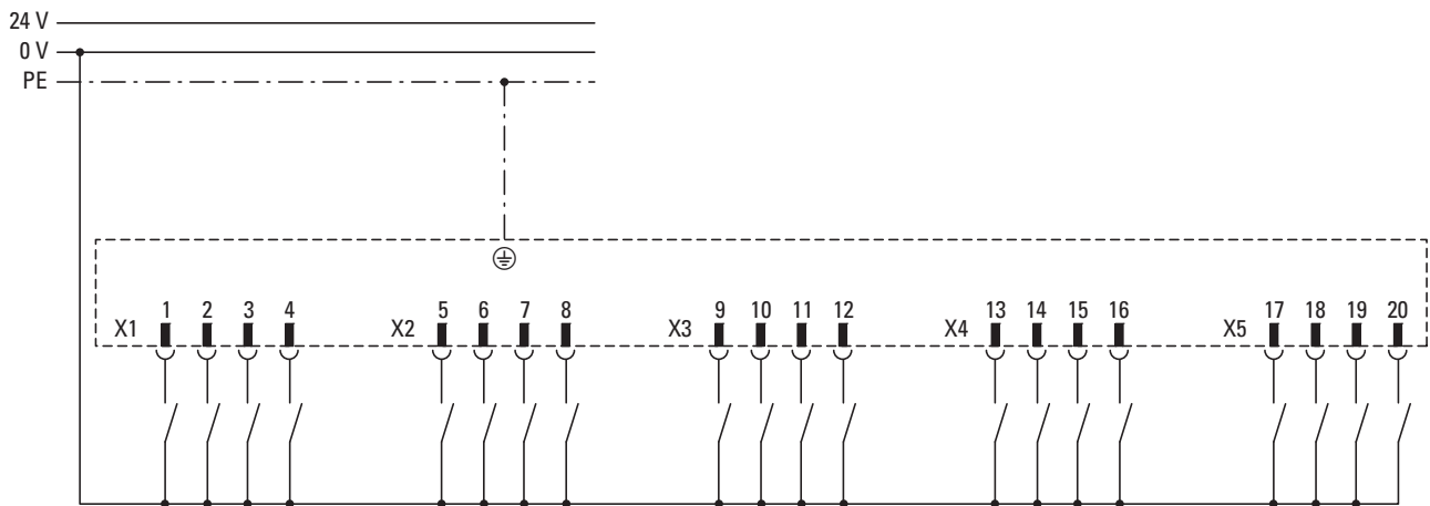
Figure 44: Input wiring
