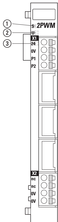
Figure 169: LED signals and pin assignment
