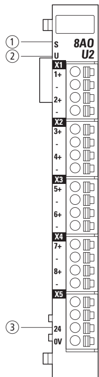
Figure 112: LED signals and pin assignment
