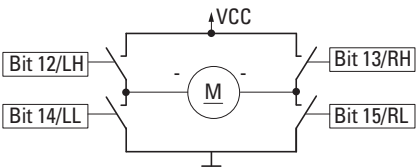
Figure 147: Block diagram showing open motor
