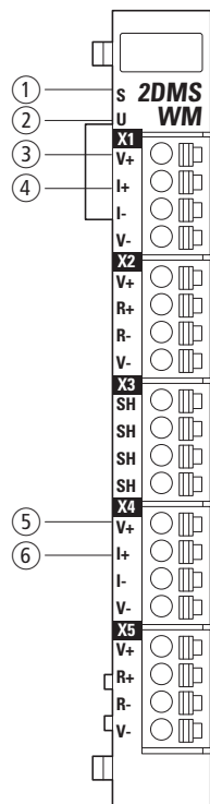
Figure 136: LED signals and pin assignment
