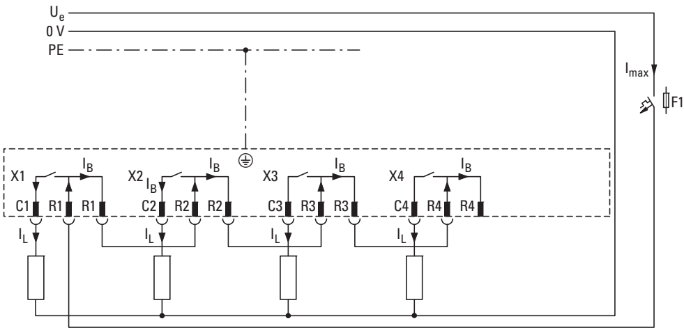
Figure 49: Wiring diagram with U_e looped through
