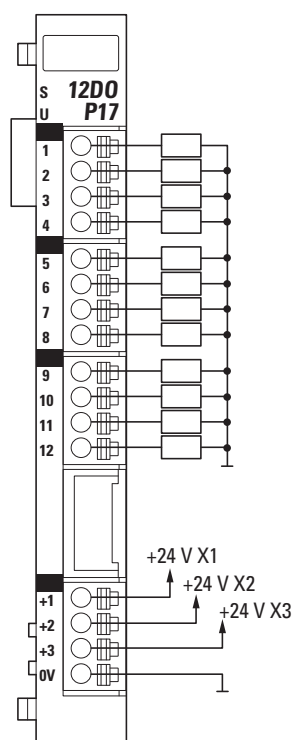
Figure 64: Wiring example
