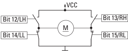
Figure 146: Block diagram showing a motor armature short-circuit
