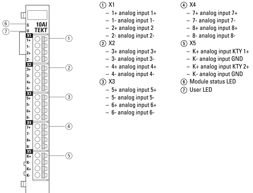
Figure 105: LED signals and pin assignment
