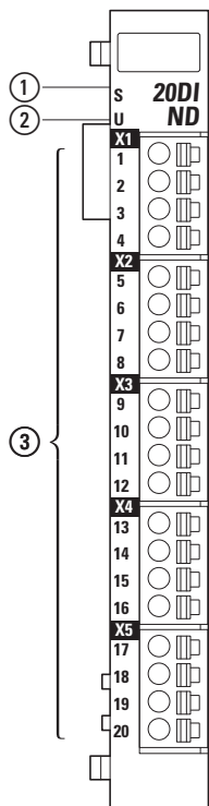
Figure 42: LED signals and pin assignment for XN-322-20DI-ND
