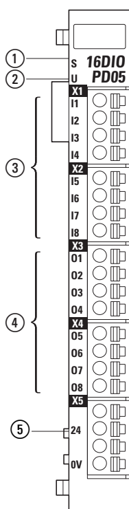
Figure 74: XN-322-16DIO-PD05 LEDs
