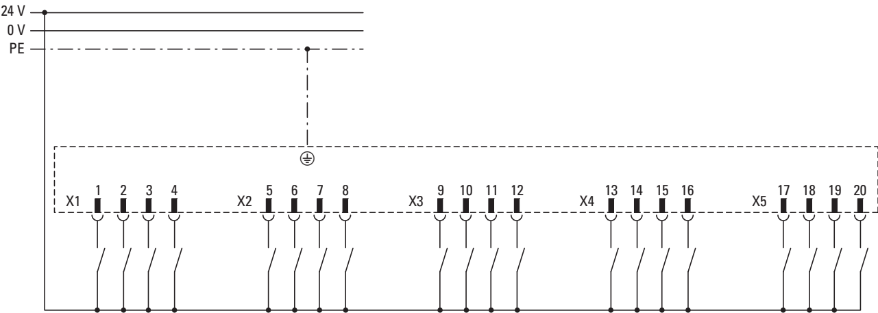
Figure 40: Input wiring
