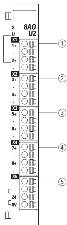
Figure 113: Pin assignment
