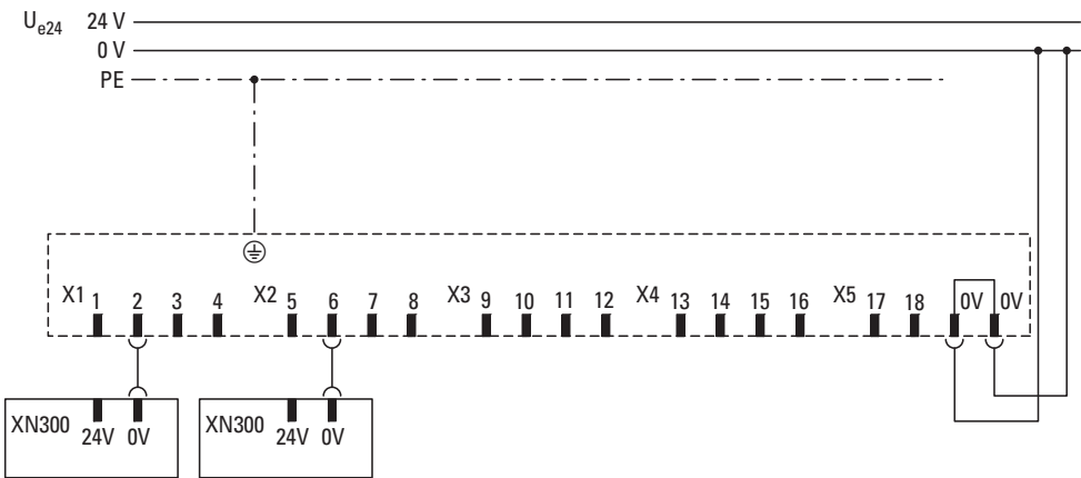
Figure 20: Wiring example
