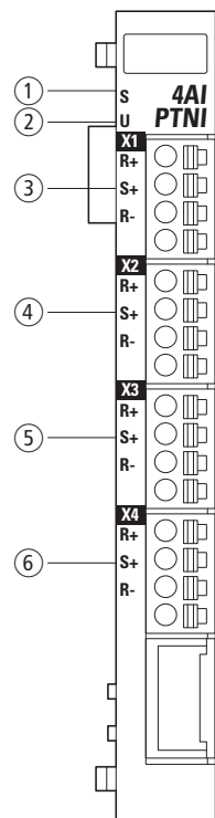
Figure 88: LED signals and pin assignment
