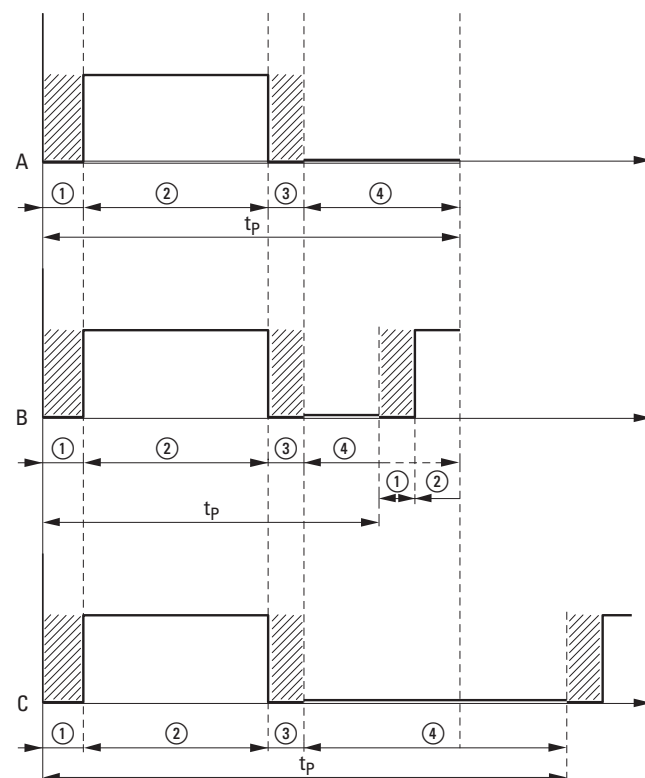
Figure 150: Output signal
