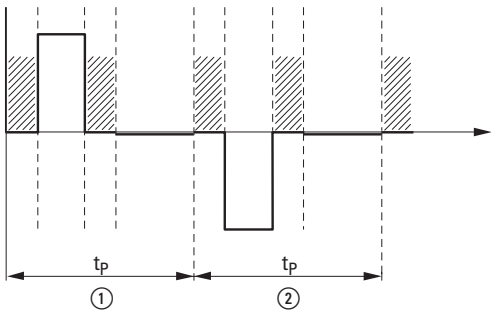
Figure 153: Pulse-width modulated signal at module output M+ for the operating direction change example ① Forward ② Counter-clockwise
