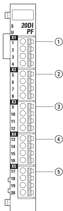
Figure 35: Pin assignment
