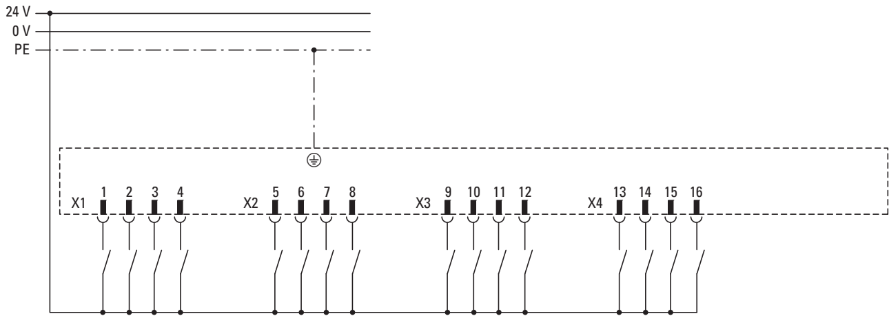
Figure 30: Input wiring
