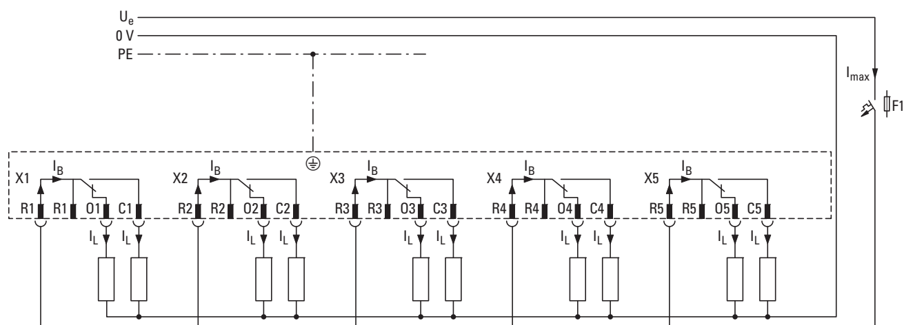
Figure 56: Wiring diagram with U_e at all five connection terminals for total currents > 10\text{ A}
