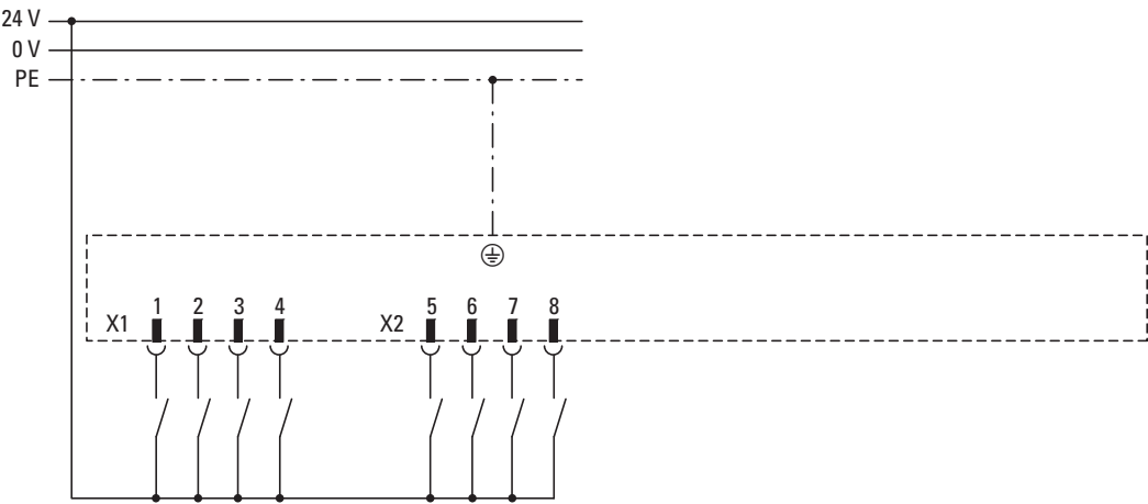
Figure 27: Input wiring
