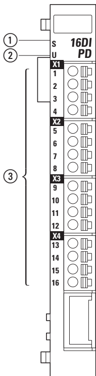
Figure 28: LED signals and pin assignment for XN-322-16DI-PD 1 Module status LED 2 User LED 3 Status LEDs for inputs 1 to 16
