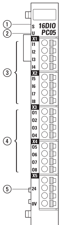
Figure 79: XN-322-16DIO-PC05 LEDs
