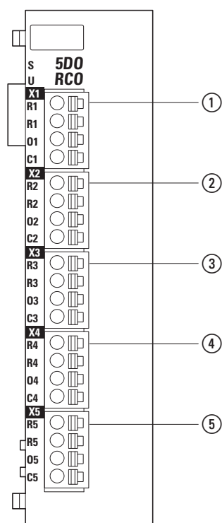
Figure 53: Pin assignment
