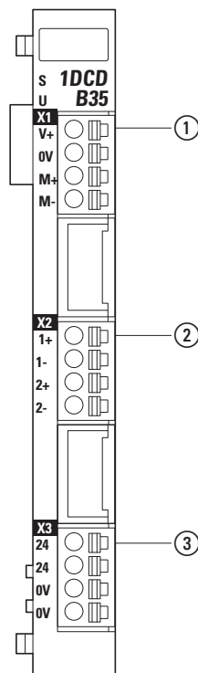
Figure 141: Pin assignment XN-322-1DCD-B35
