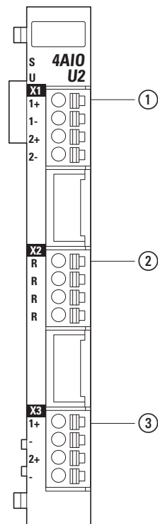
Figure 117: Pin assignment
