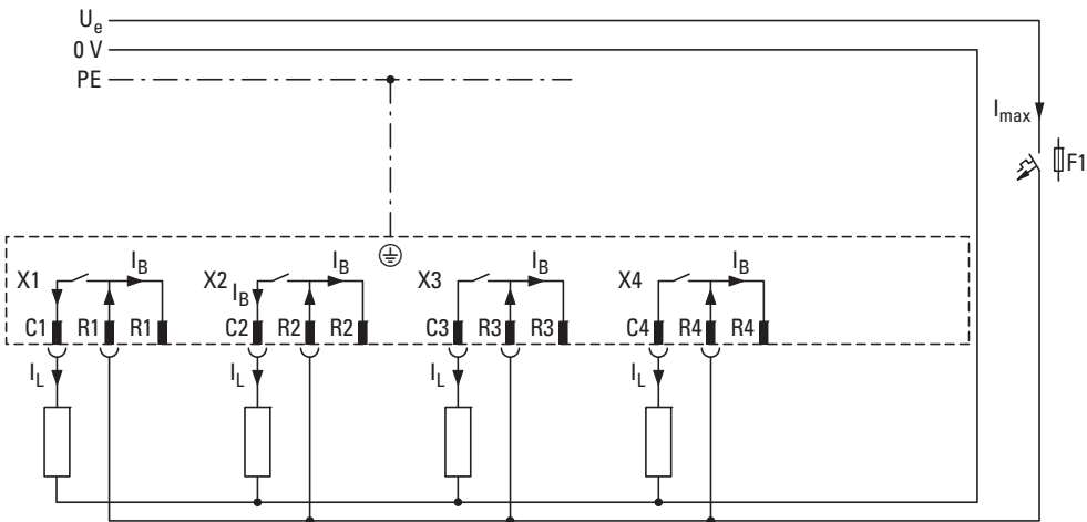
Figure 50: Wiring diagram with U_e at all four connection terminals for total currents > 10 A
