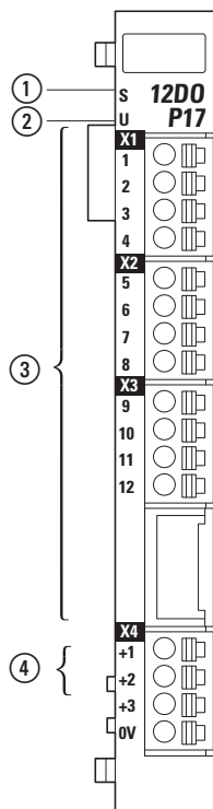
Figure 62: LED signals and pin assignment
