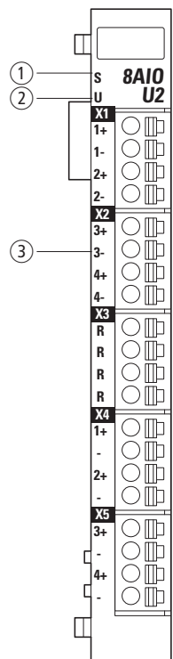
Figure 122: LED signals and pin assignment
