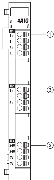
Figure 129: Pin assignment
