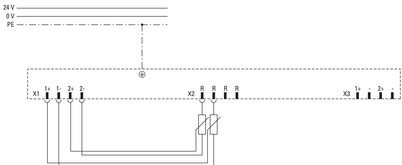
Figure 119: Potentiometer measurement wiring
