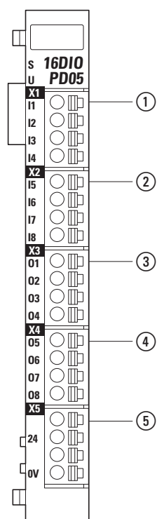
Figure 75: Pin assignment
