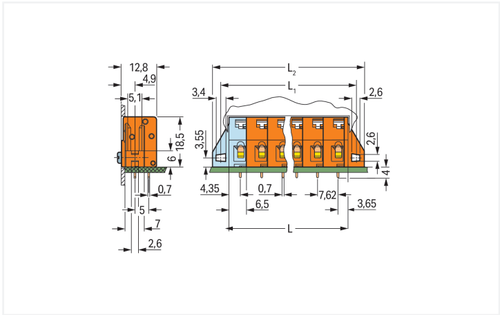
Dimensions in mm L = (\text{pole no.} - 1) \times \text{pin spacing} + 6.5 \text{ mm} + 1.5 \text{ mm} L_1 = L + 5.8 \text{ mm} L_2 = L_1 + 6 \text{ mm}
