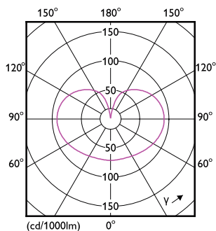
Light Distribution Diagram - MAS VLE LEDBulbD3.4-40W E27 940 A60FR G
