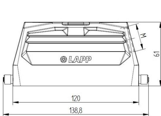
Side cable entry
