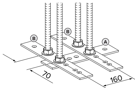
Fig. 2: Dimensions [mm]
