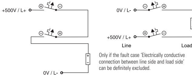
Connection example at 500 V=, 2-pole
