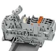
Pivoting double-deck marker carrier (2002-121) and 2-conductor disconnect/test terminal block (2002-1671)
