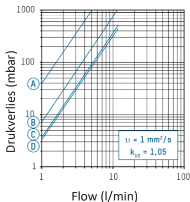
223.7702.000 (DN 20 | 1" | 1...12 l/min)
