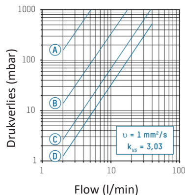
223.7704.000 (DN 20 | 1" | 2...40 l/min)
