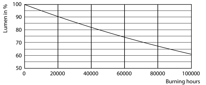
Lumen Maintenance Diagram - MAS LED SON-T EM 6Klm 34W 740 E27
