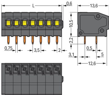
Dimensions in mm L = (pole no. x pin spacing) + 1.5 mm
