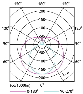
Light Distribution Diagram - MAS LEDtube VLE 1500mm 19.3W/23W 830 T8
